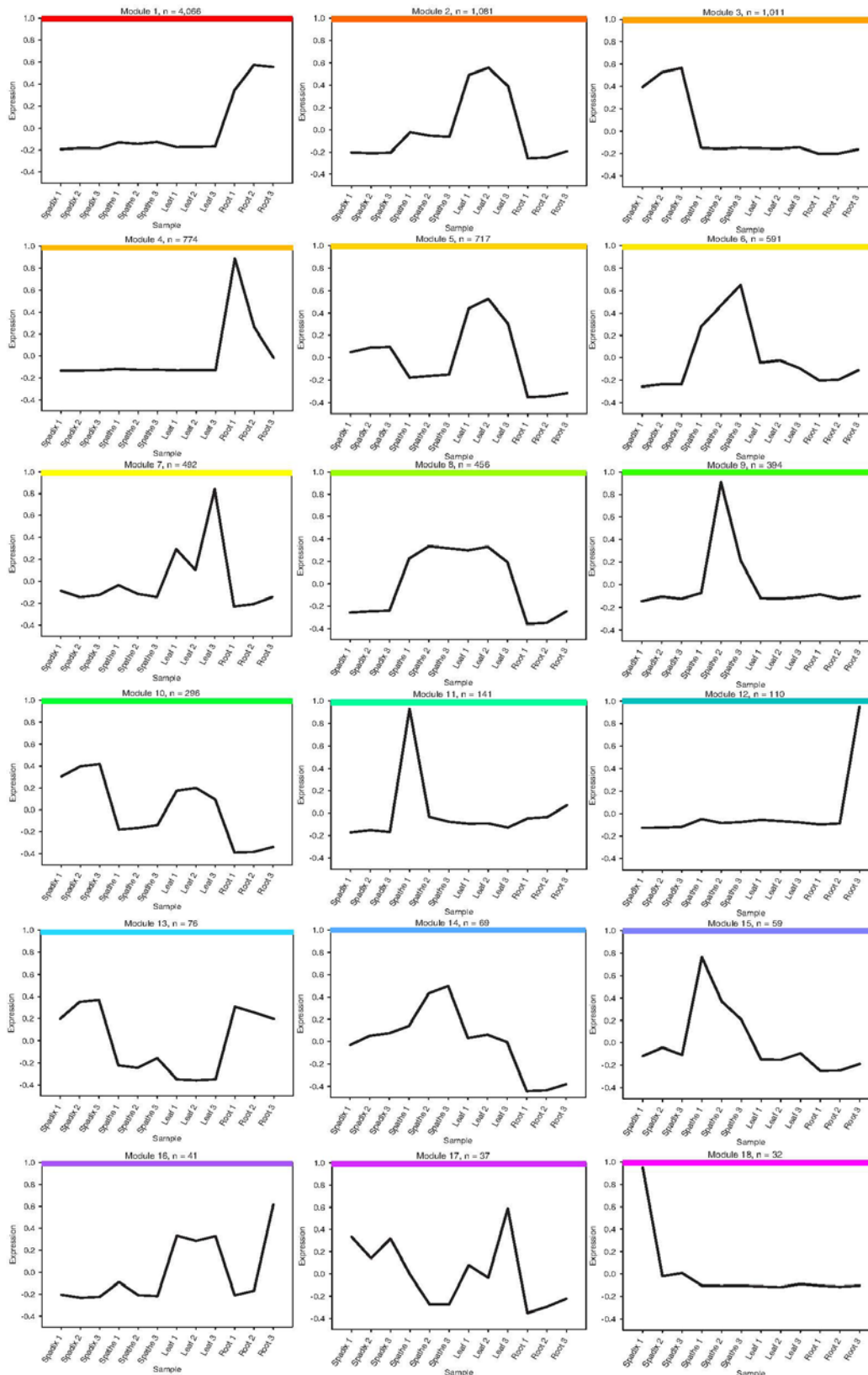
Supplementary Figure S2 – Network co-expression module profiles. Organ specific expression profiles for the 18 co-expression modules in Fig. 7. The colored bar above each plot corresponds to the module color found in Fig. 7 and the number of genes (n) are included at the top of each plot.
