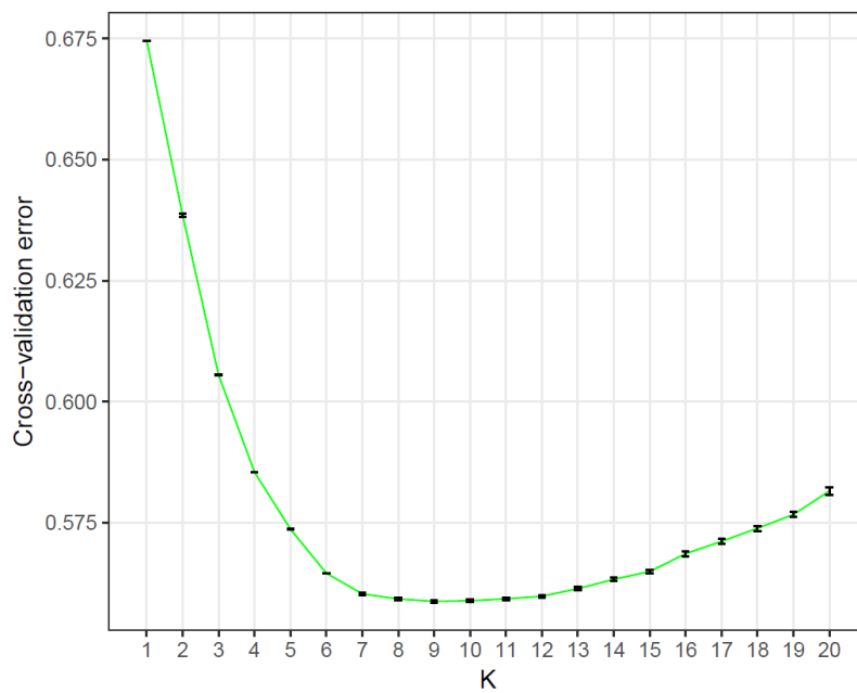
S2 Fig. Cross-validation (CV) error and standard error of ADMIXTURE runs of K ranging from 1 to 20. The lowest CV error was K = 9 .
