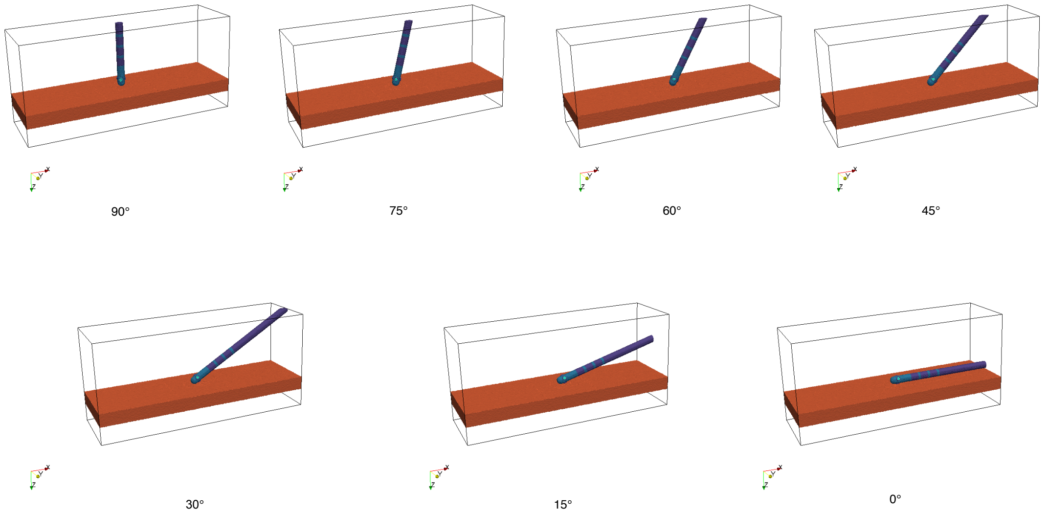
SUPPLEMENTARY FIGURE 1: Varying tilting angle between catheter and healthy myocardium between 90° and 0°. The excitation wavefront is propagating from the left tissue boundary (electrical activity is not shown here).
