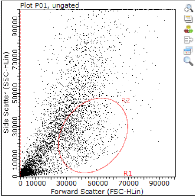
300,000 particles/cell
