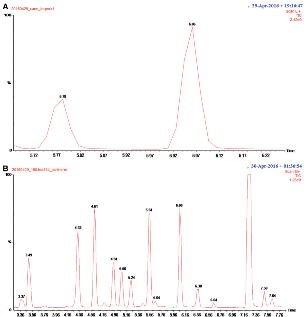
SUPPLEMENTARY FIG. S1. GC-MS chromatograms and mass spectra of cis -ocimene and trans -ocimene in reference mix and representative Jack Herer sample. (A) Ocimene peaks in CannTerpMix 1 ( cis -ocimene 5.78 min, trans -ocimene 6.06 min). (B) Representative Jack Herer sample with \alpha -phellandrene 4.94 min, 3-carene 5.06 min, \alpha -terpinene, 5.24 min, and trans -ocimene 6.06 min. (C) Mass spectrum of cis -ocimene standard. (D) Mass spectrum of trans -ocimene standard. (E) Mass spectrum of trans -ocimene in Jack Herer sample. GC-MS, gas chromatography–mass spectrometry.
