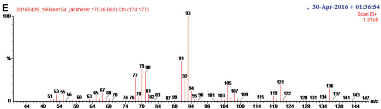
SUPPLEMENTARY FIG. S1. (Continued).
