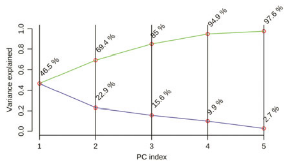
SUPPLEMENTARY FIG. S2. Principal component total variance explained (green line) and individual component variation explained (blue line).
