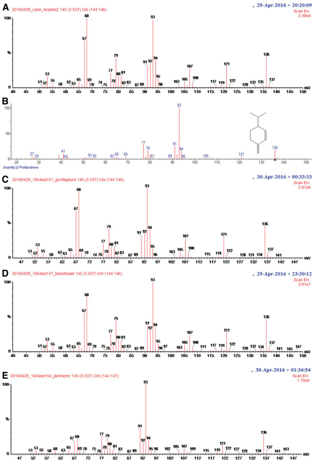
SUPPLEMENTARY FIG. S3. (A) Mass spectrum of limonene in CannTerpMix 2. (B) Mass spectrum of \beta -phellandrene in NIST library Version 2.0. (C) Limonene peak in a sample of Gorilla Glue #4. (D) Limonene peak in a sample of Blue Dream. (E) Peak containing \beta -phellandrene overlapping with limonene in Jack Herer sample.
