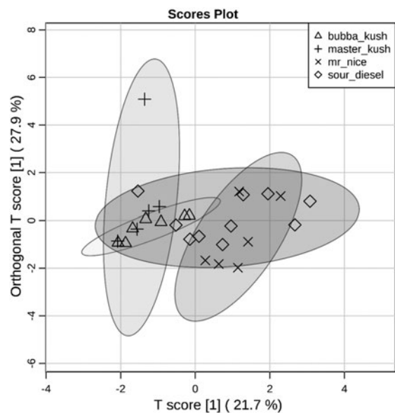
SUPPLEMENTARY FIG. S4. OPLS-DA analysis of bisabolol group with cultivar names as classes. OPLS-DA, orthogonal partial least squares discriminant analysis.
