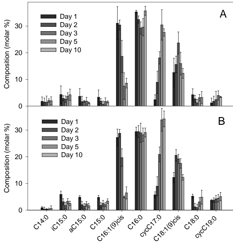
Figure S3: Composition (molar percentage) of C. necator JMP134 FAME profiles in the control (upper) and sand (lower) samples at each sampling date. Error bars correspond to the standard deviation calculated for 3 replicates.
