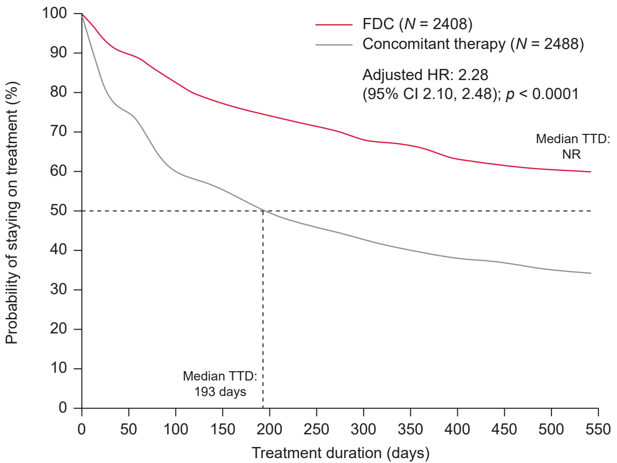
Figure S3. Median time to discontinuation in any FDC* compared with any concomitant therapy*. * \alpha -blocker plus an antimuscarinic or 5-ARI. 5-ARI: 5 \alpha -reductase inhibitor; CI: confidence intervals; FDC: fixed-dose combination; HR: hazard ratio; NR: not reached; TTD: time to discontinuation
