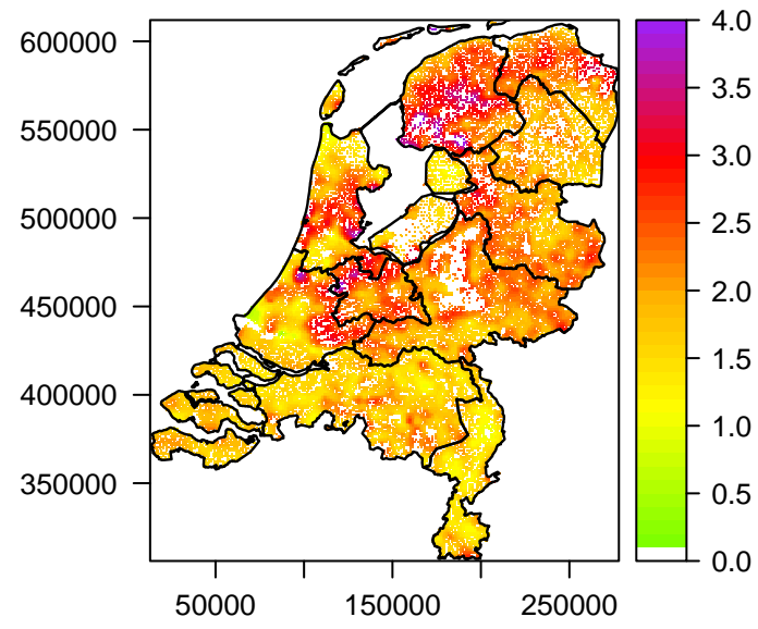
Mean LAI [ m 2 /m 2 ] per km 2 (2009 – 5)
