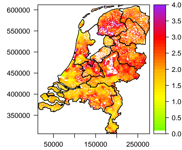
Mean LAI [ m 2 /m 2 ] per km 2 (2009 – 7)
