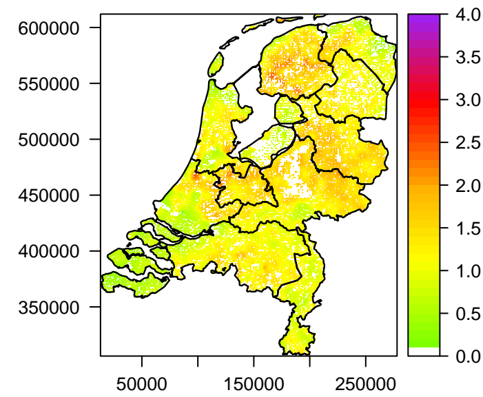
Mean LAI [ m 2 /m 2 ] per km 2 (2009 – 11)
