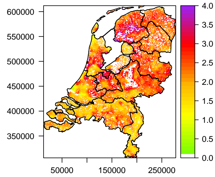
Mean LAI [ m 2 /m 2 ] per km 2 (2009 – 6)
