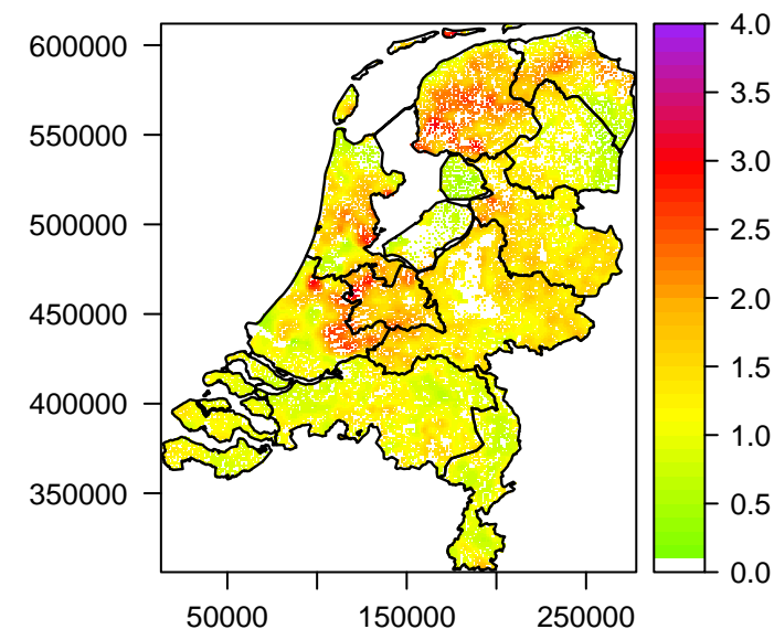
Mean LAI [ m 2 /m 2 ] per km 2 (2009 – 3)
