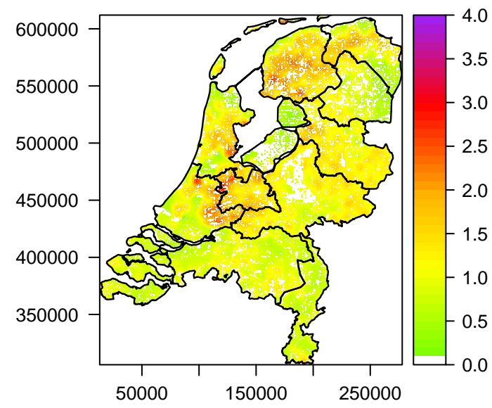
Mean LAI [ m 2 /m 2 ] per km 2 (2009 – 2)
