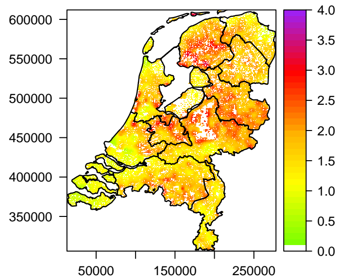
Mean LAI [ m 2 /m 2 ] per km 2 (2009 – 9)
