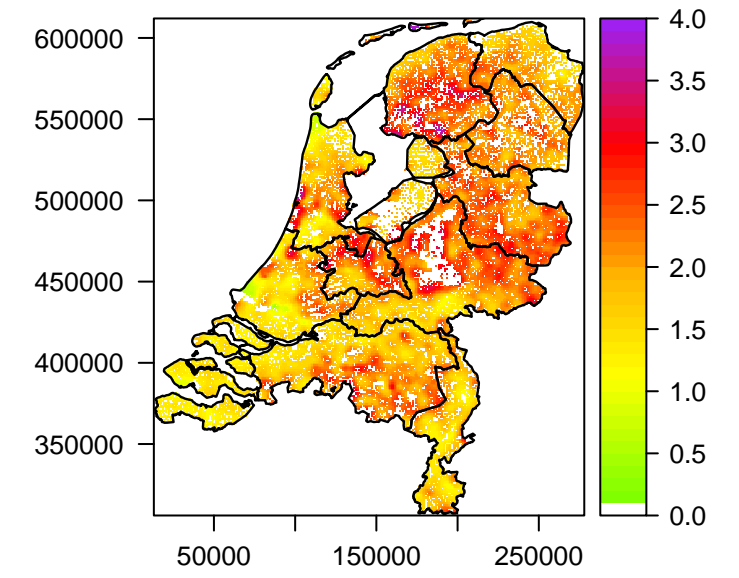
Mean LAI [ m 2 /m 2 ] per km 2 (2009 – 8)
