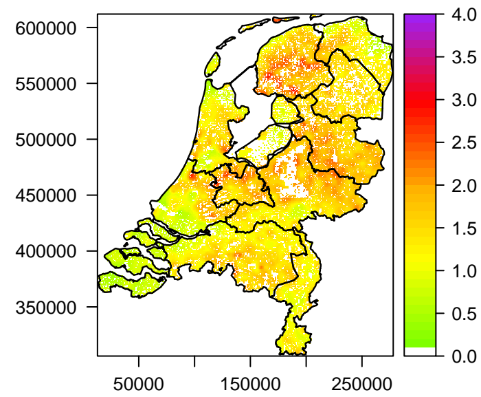
Mean LAI [ m 2 /m 2 ] per km 2 (2009 – 10)
