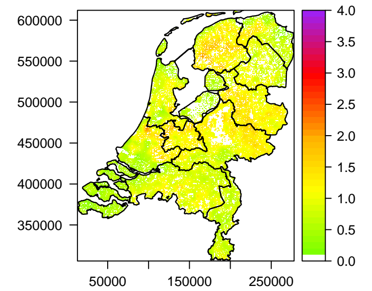
Mean LAI [ m 2 /m 2 ] per km 2 (2009 – 12)
