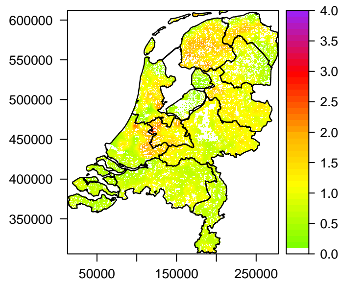
Mean LAI [ m 2 /m 2 ] per km 2 (2009 – 1)
