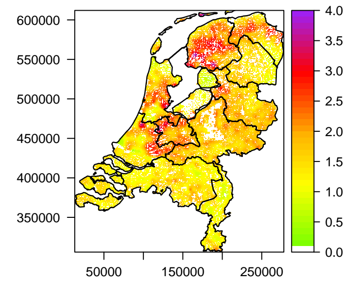
Mean LAI [ m 2 /m 2 ] per km 2 (2009 – 4)
