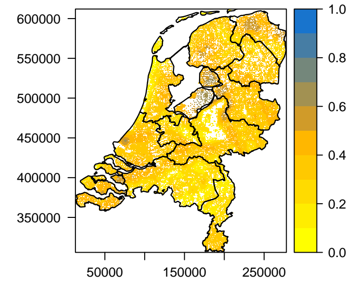
Mean SM [%] per km 2 (2009 – 7)
