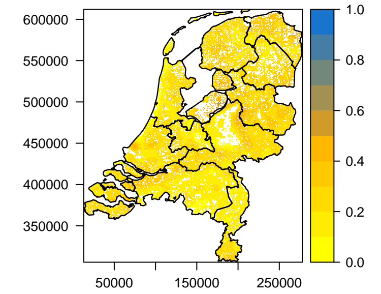
Mean SM [%] per km 2 (2009 – 8)
