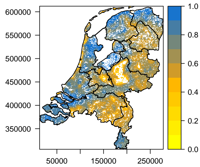
Mean SM [%] per km 2 (2009 – 1)
