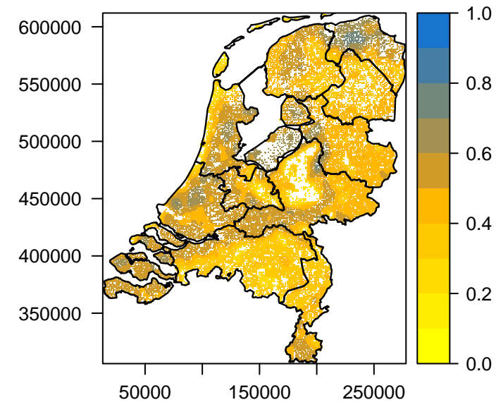
Mean SM [%] per km 2 (2009 – 10)
