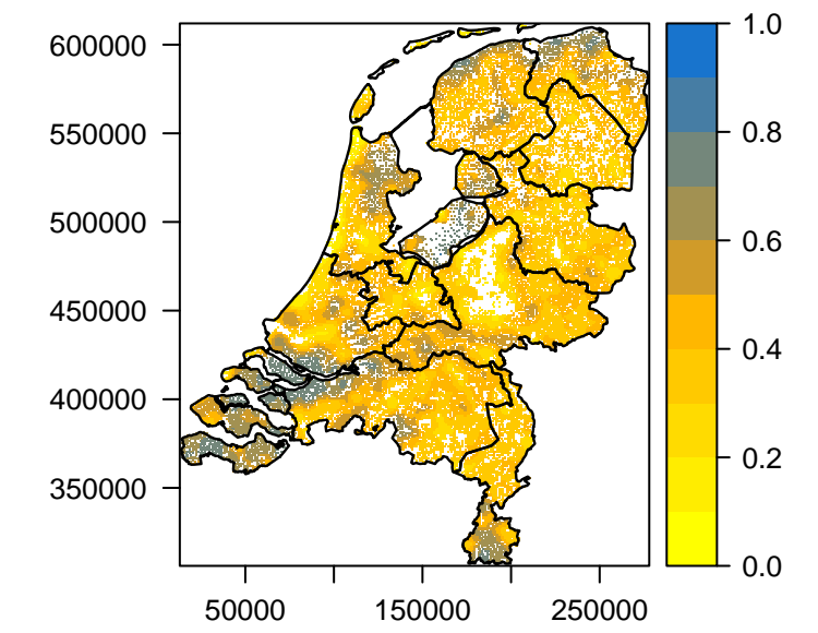
Mean SM [%] per km 2 (2009 – 4)
