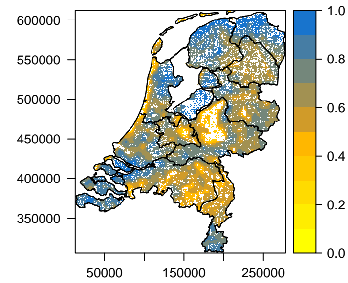
Mean SM [%] per km 2 (2009 – 3)
