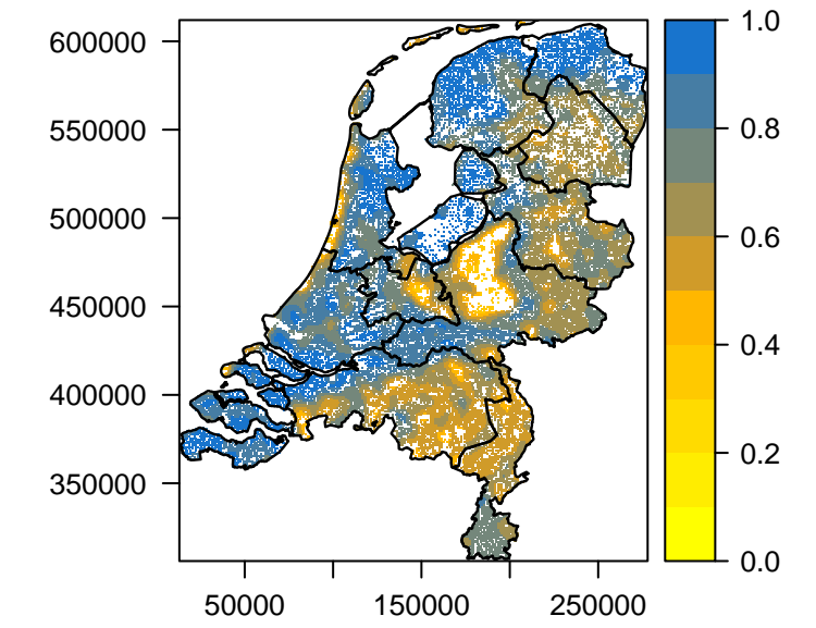
Mean SM [%] per km 2 (2009 – 12)
