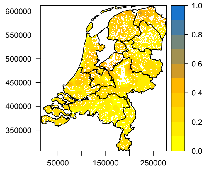
Mean SM [%] per km 2 (2009 – 9)
