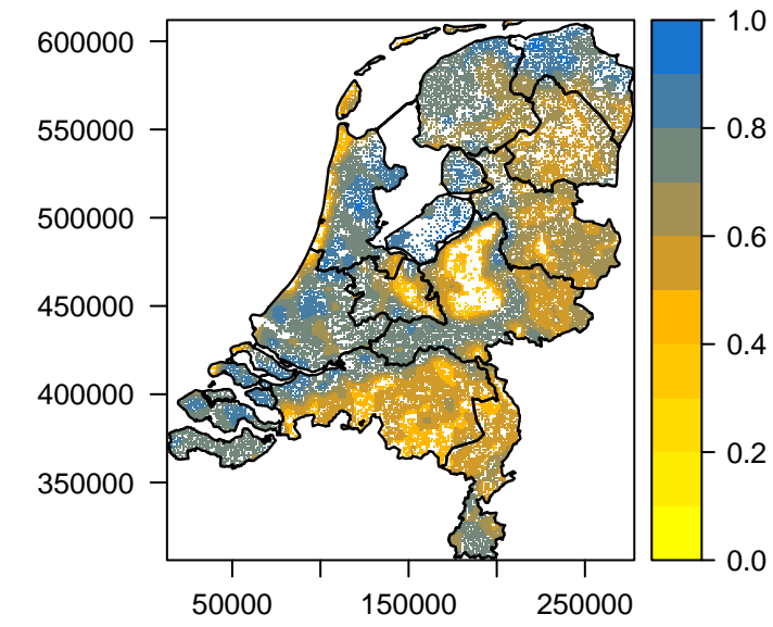
Mean SM [%] per km 2 (2009 – 11)
