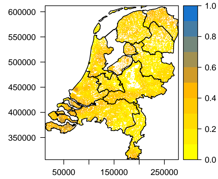
Mean SM [%] per km 2 (2009 – 6)
