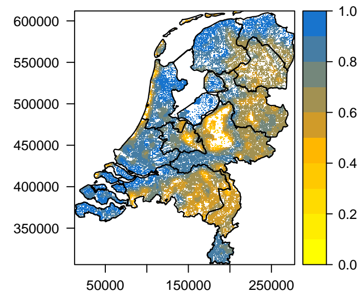
Mean SM [%] per km 2 (2009 – 2)
