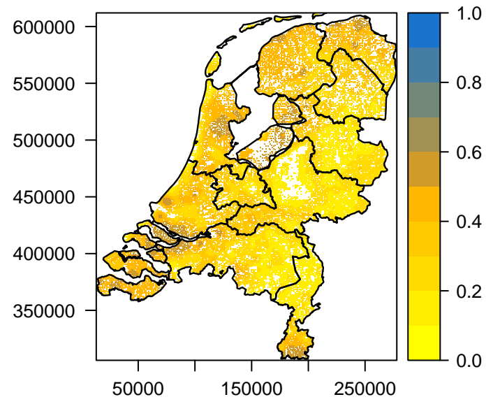
Mean SM [%] per km 2 (2009 – 5)
