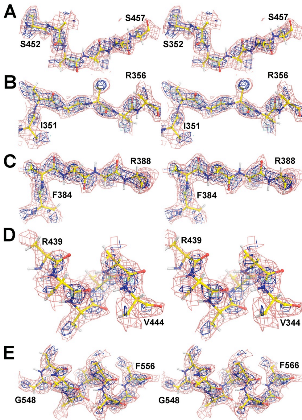
Figure S2. Sreodiagram continued from Figure 2 in three contour levels (+7 \sigma , cyan; +5 \sigma , blue, and +3 \sigma , salmon)
