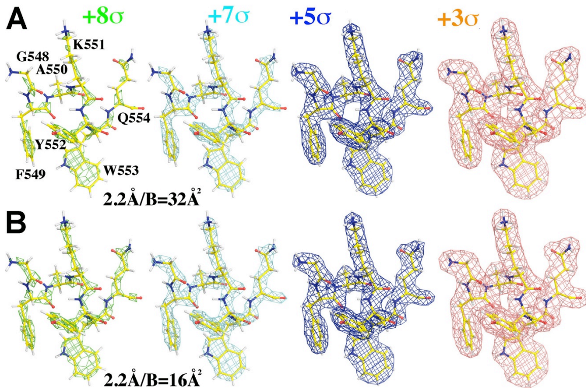
Figure S1. Simulated ESP map using neutral atomic models with B=32\text{\AA}^2 (A) or B=16\text{\AA}^2 (B) contoured at +8.0\sigma (green) as well as three contour levels used in Figure 2, namely, +7\sigma (cyan), +5.0\sigma (blue), and +3.0\sigma (salmon).
