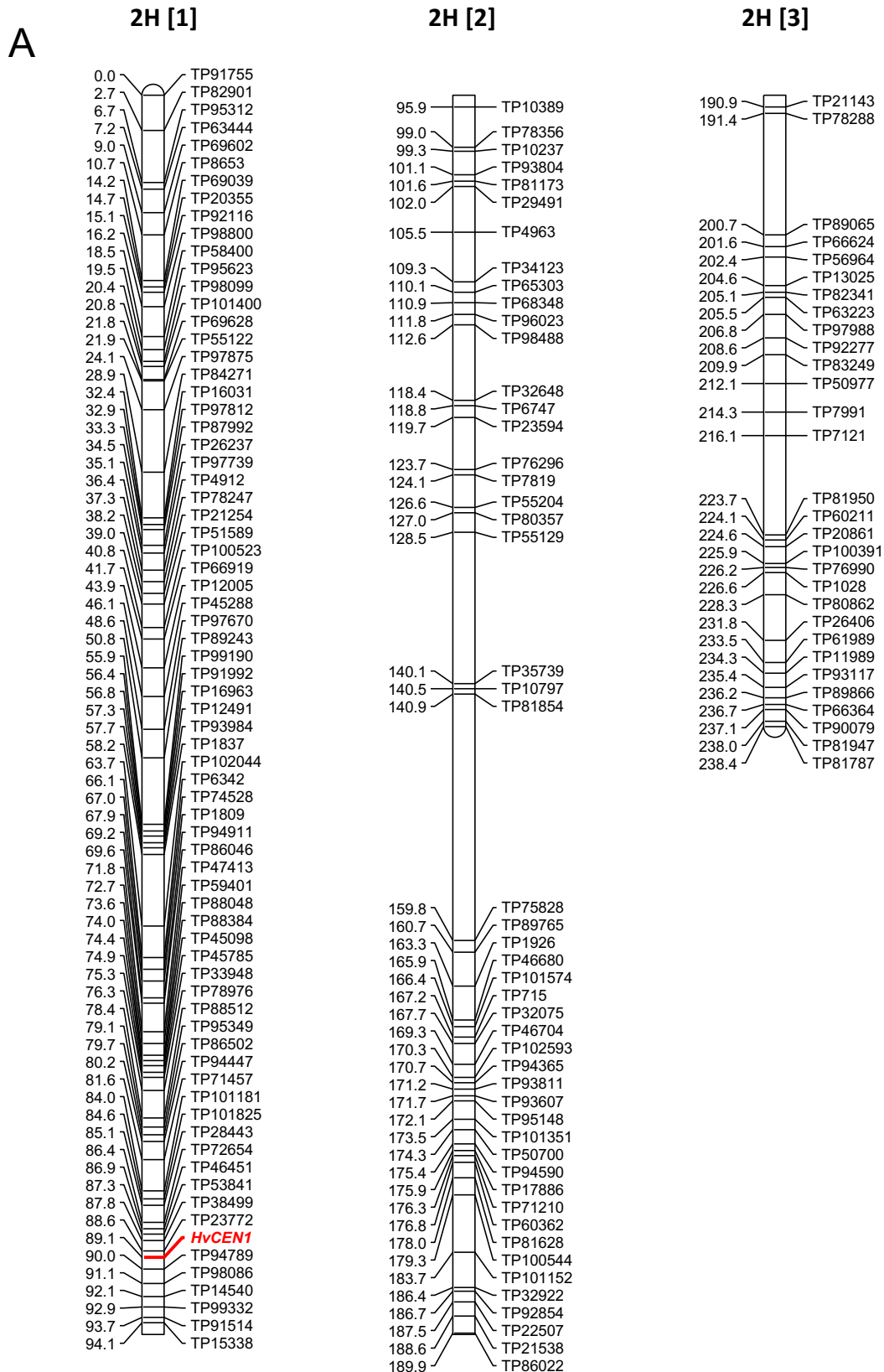
S2 Fig. Genetic map of chromosome 2H in the CW (A) and FW (B) populations.
