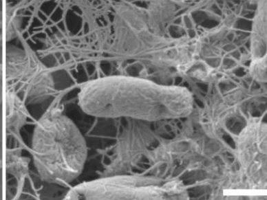
NCR169pl 8.4
