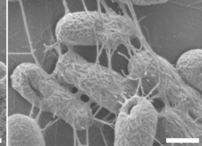
NCR124 pl 6.9
