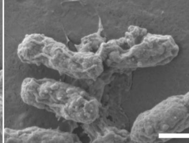
NCR280 pl 9.8
