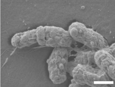
NCR032 pl 9.8
