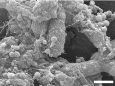
NCR247 pl 10.1
