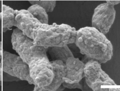
NCR044 pl 10.6
