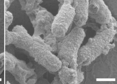
NCR183 pl 10.1
