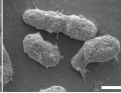
NCR192 pl 9.7
