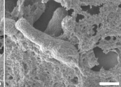
NCR057 pl 8.9
