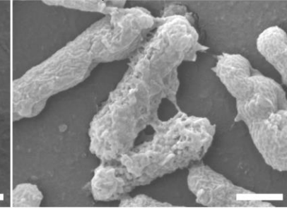
NCR147 pl 9.7
