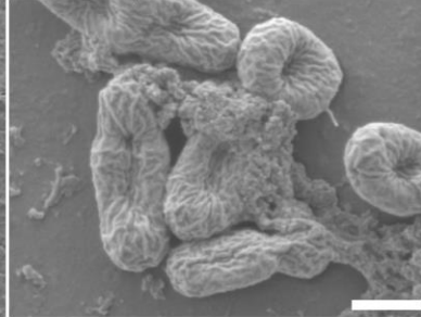
NCR121pl 6.7
