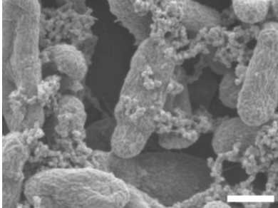
NCR200pl 8.3
