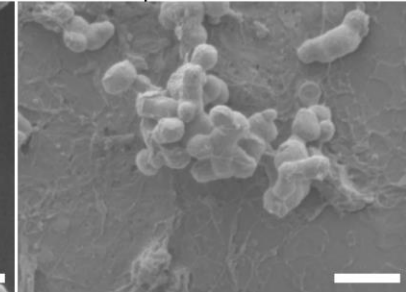
NCR335 pl 11.2
