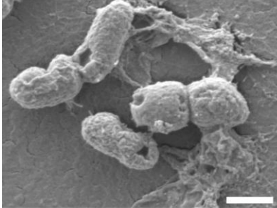
NCR084pl 6.7
