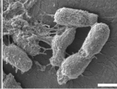
NCR209pl 4.5
