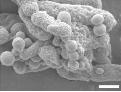
NCR137 pl 9.7
