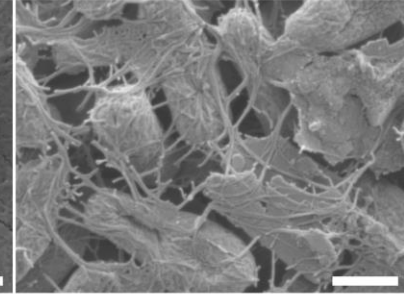
NCR001 pl 5
