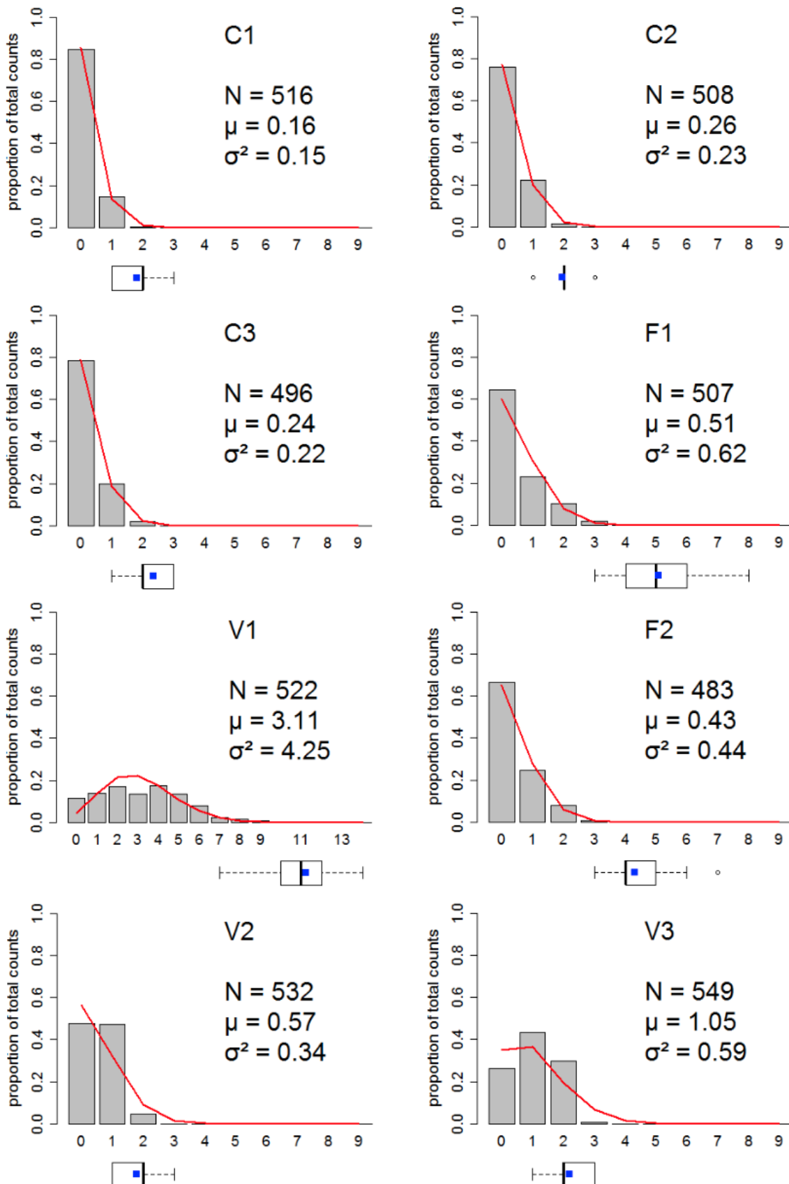
Figure S2: Protrusion frequency per segment; N =number of segments analyzed, \mu =mean, \sigma^2 =variance: the predicted Poisson distribution is shown in red. Box plots show cell counts along the edge of each segment (taken from a representative sample of 10 micro-patterns)..
