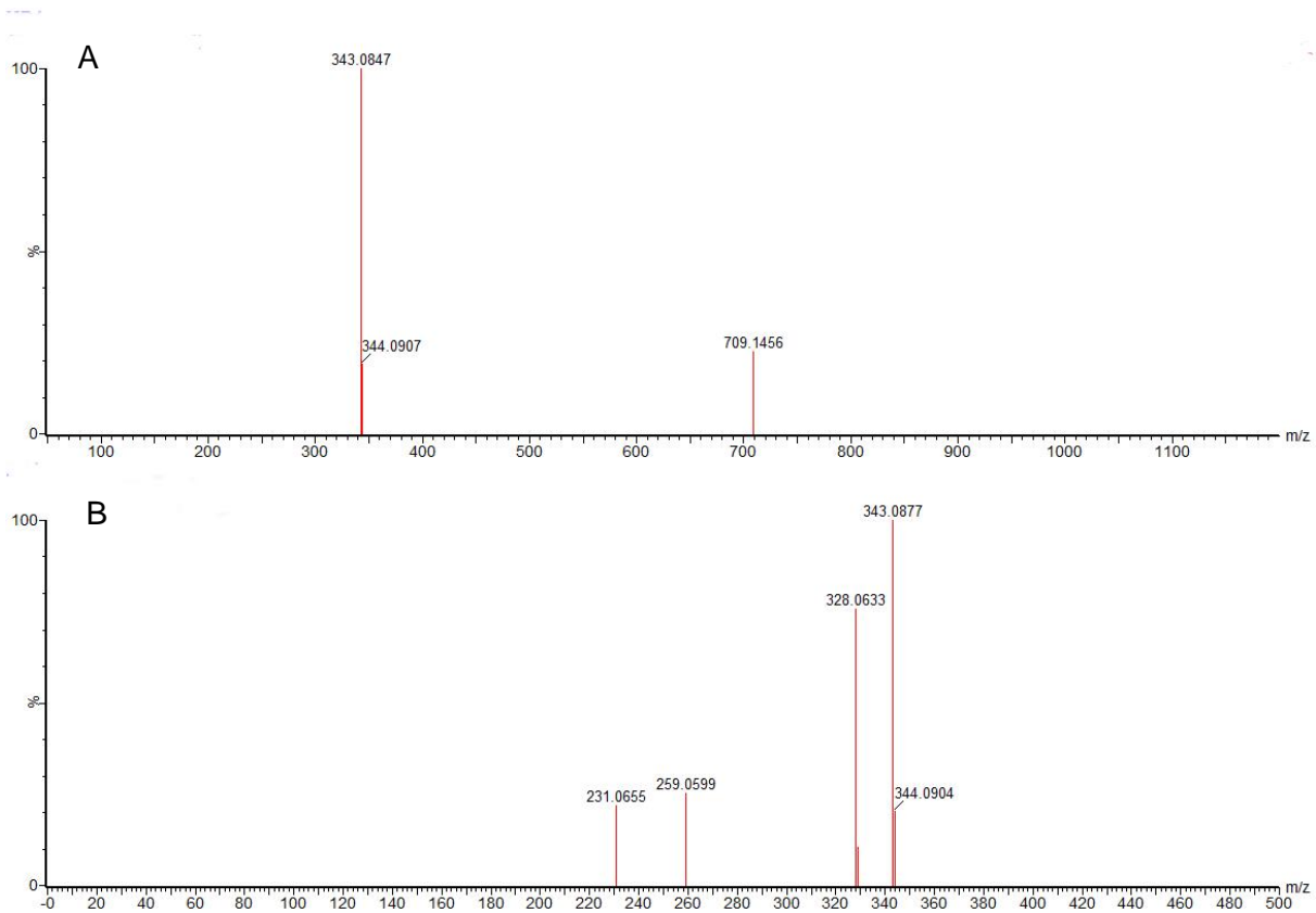
S3 Fig. MS and MS 2 spectra of usnic acid in one chemotype of the lichen Montanelia disjuncta . (A) MS spectrum of usnic acid 4 showing the adduct ion at m/z 709.1456 and molecular ion at m/z 343.0847. (B) MS 2 spectrum of the usnic acid molecular ion.
