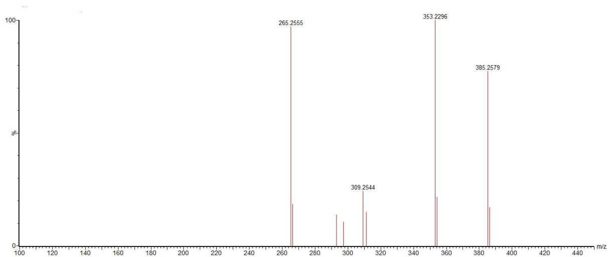
S4 Fig. MS 2 spectrum of rangiformic acid.
