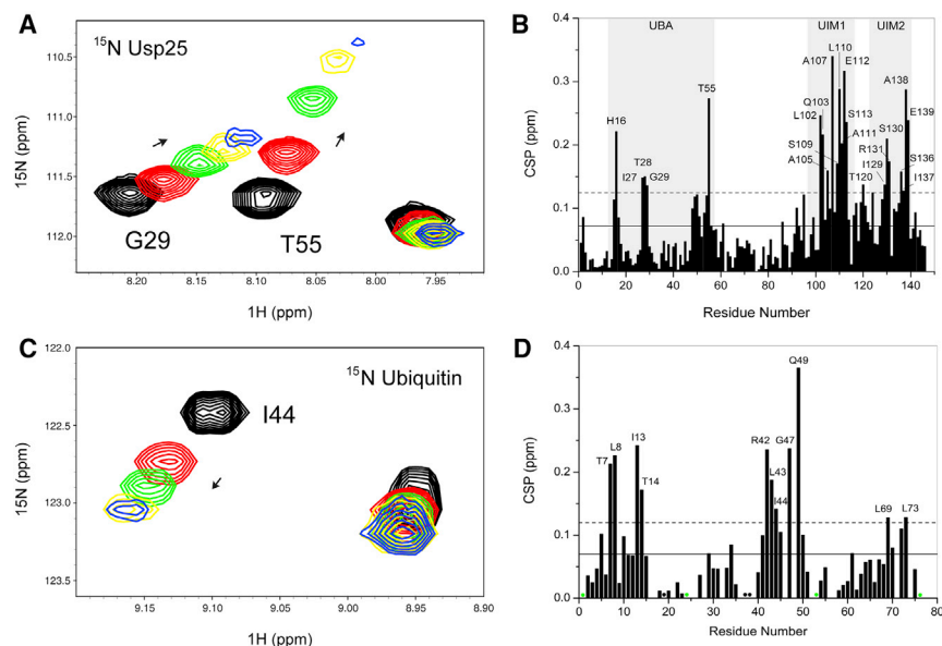
FIGURE 2 Characterization of the interaction between the Usp25 UBR and monoubiquitin. (A) Zoomed view of the superimposed ^1\text{H} - ^{15}\text{N} HSQC spectra for the ^{15}\text{N} -labeled Usp25 UBR titrated with monoubiquitin at Usp25 UBR/monoubiquitin molar ratios of 1:0 (black), 1:5 (red), 1:10 (green), 1:20 (yellow), and 1:30 (blue). (B) CSP analysis for the Usp25 UBR upon its binding to monoubiquitin. (C) Zoomed view of the superimposed ^1\text{H} - ^{15}\text{N} HSQC spectra for ^{15}\text{N} -labeled monoubiquitin titrated with Usp25 UBR at monoubiquitin/Usp25 UBR molar ratios of 1:0 (black), 1:1 (red), 1:2 (green), 1:5 (yellow) and 1:10 (blue). (D) CSP analysis for monoubiquitin upon its binding to Usp25 UBR. Green dots indicate residues that were undetectable and black dots represent proline residues. Solid and dashed lines in (B) and (D) are indicators for the mean and mean + SD values, respectively. Residues with CSP values greater than the mean + SD value are labeled. To see this figure in color, go online.
