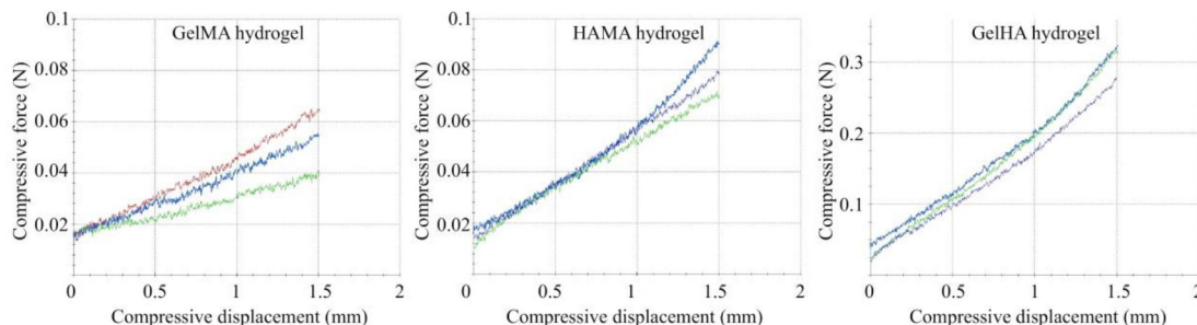
Supplementary Figure 1: Load-displacement curves of the hydrogels.
