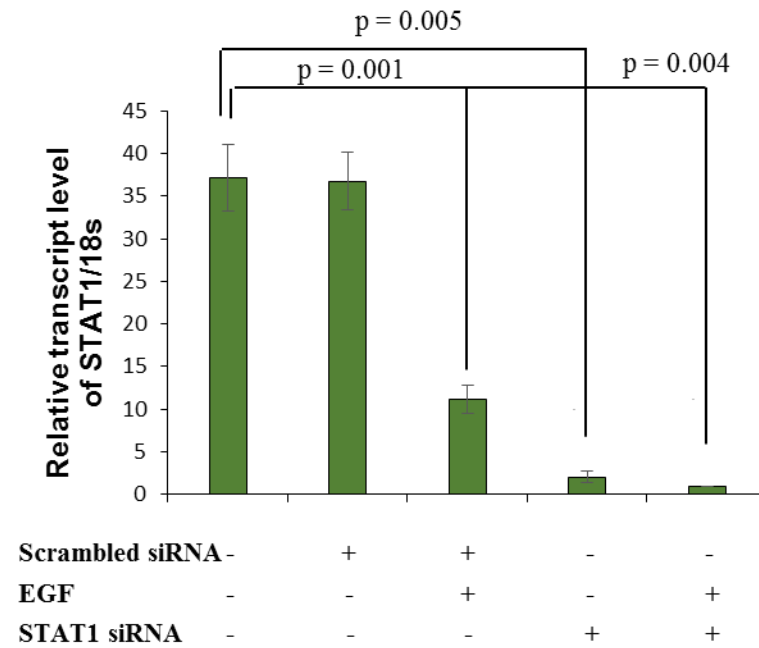
S4 Fig: Transcript levels of STAT1 after silencing. Bar graph represents transcript levels of STAT1 mRNA by qRT-PCR in naïve, scrambled and STAT1 siRNA transfected cells either in presence or absence of EGF.
