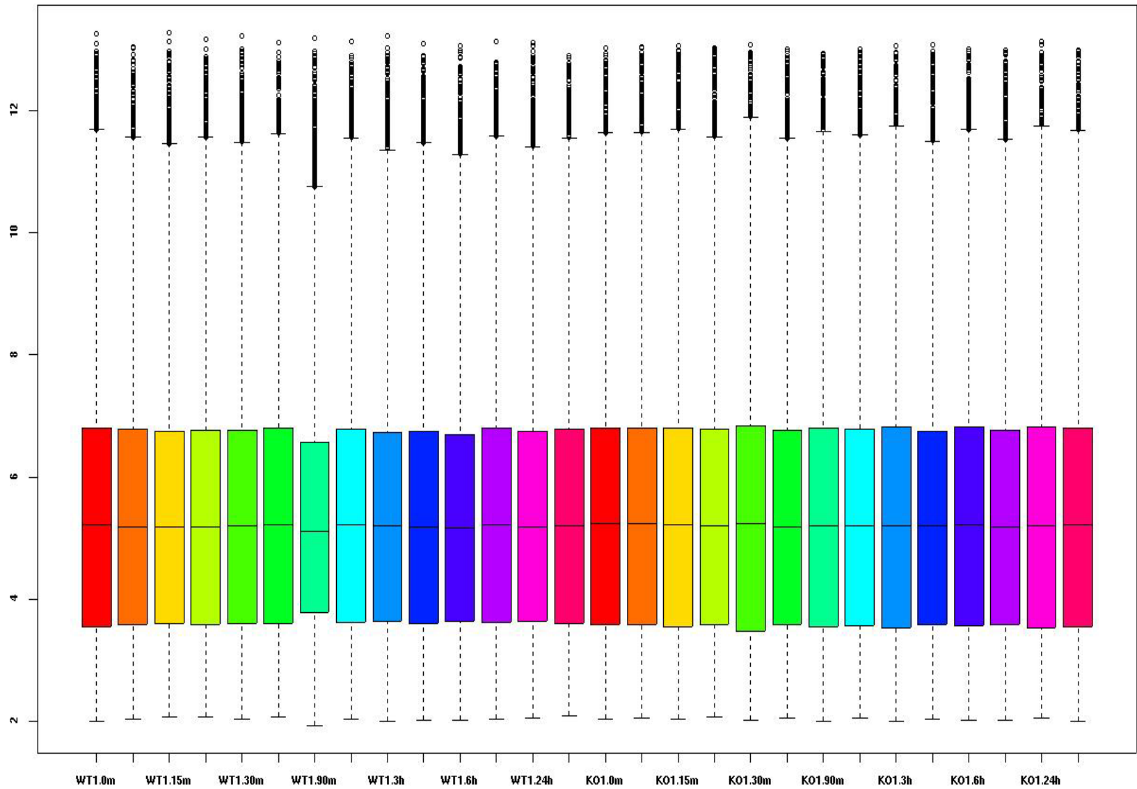
Boxplot of RMA values of All 28 Arrays
