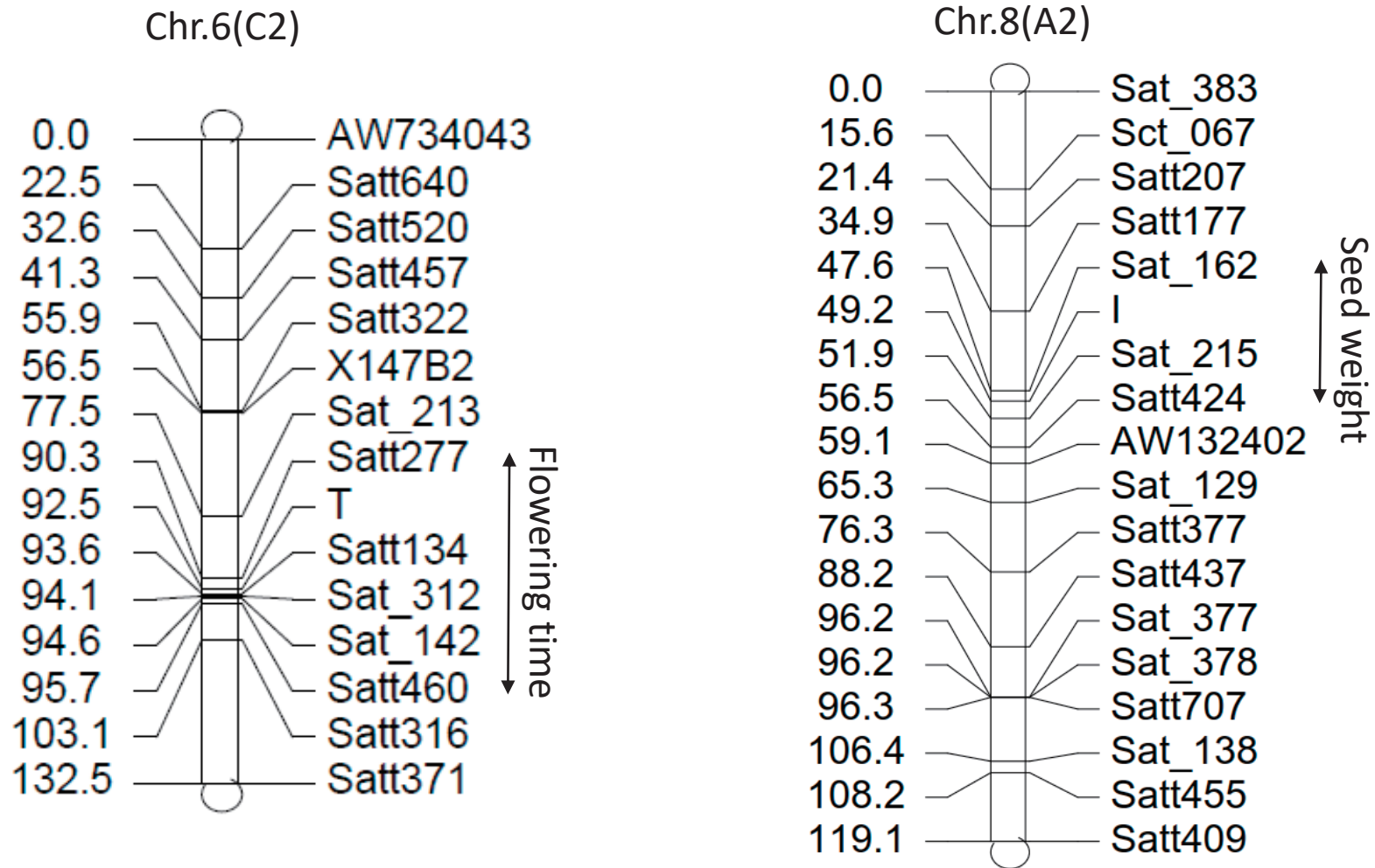
Supplemental Fig.1. Genomic locations of QTL for flowering time and seed weight.
