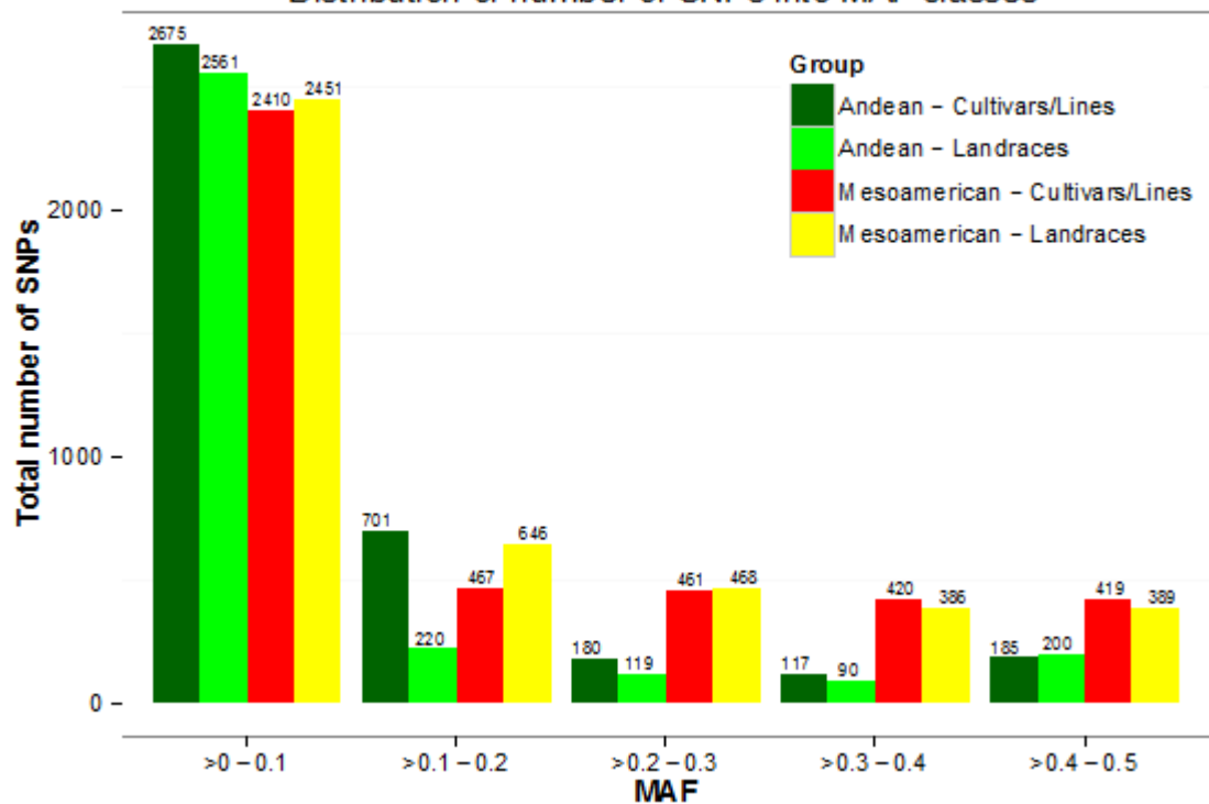
Distribution of number of SNPs into MAF classes
