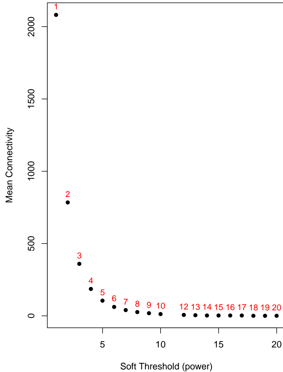
Mean connectivity
