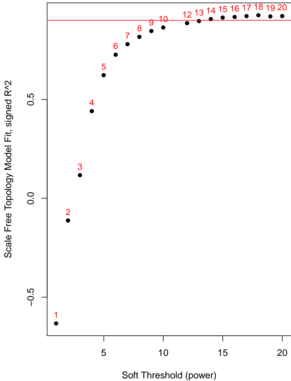
Scale independence
