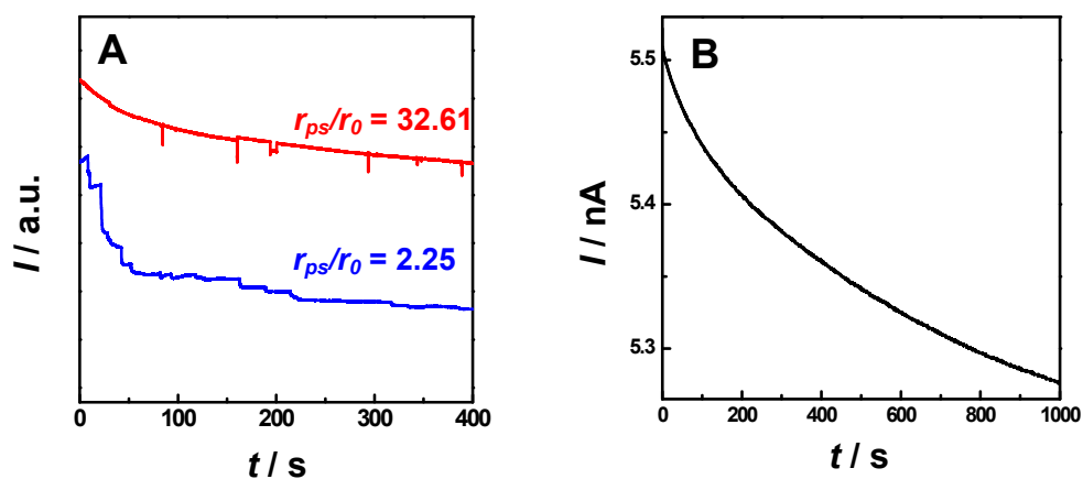
Fig. S2. (A) Typical i - t traces for 16.9 fM 2.25- \mu m-radius PS particles in 0.1 M KCl solution with different radius nanopipets: r_0 = 69 nm, r_{ps}/r_0 = 32.61 (red curve); r_0 = 1 \mu m, r_{ps}/r_0 = 2.25 (blue curve). (B) i - t response in 0.1 M KCl solution in the absence of PS particles. The applied potential was 0.2 V. The data acquisition time was 10 ms.
