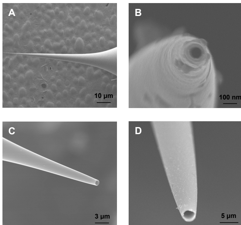
Fig. S1. SEM images of typical glass nanopipets. (A) For type A nanopipet; (B) Enlarged tip of (A); (C) and (D) For type B nanopipets of different polishing extents.
