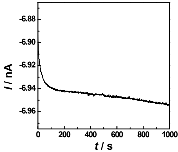
Fig. S8. i-t reponse for 16.9 fM 2.25- \mu m-radius PS particles suspended in 0.1 M KCl solution in the presence of 69-nm-radius nanopipet at -0.2 V. The data acquisition time was 10 ms.
