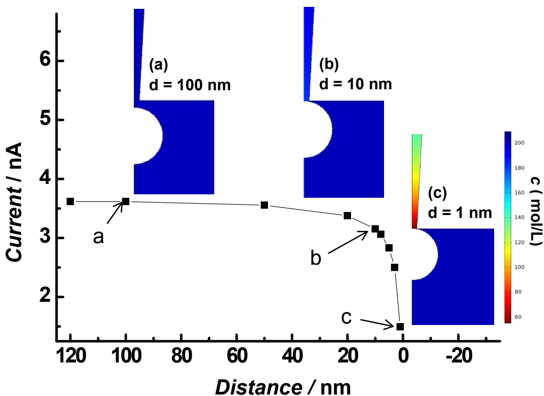
Fig. S4. Simulated current in 0.1 M KCl solution by placing a 375-nm-radius PS particle at different distance from the orifice of a 69-nm-radius nanopipet. Inset profiles represent concentration distribution of electrolyte solution at different distance from the orifice to the particle.
