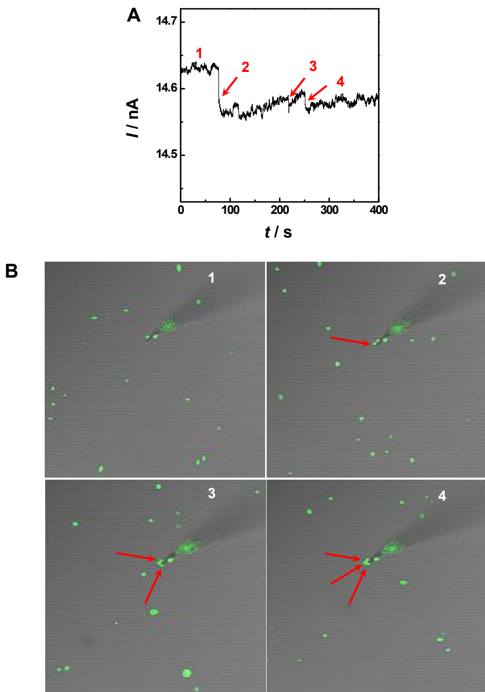
Fig. S6. (A) Representative current transient recorded with a 69-nm-radius nanopipet in 0.1 M KCl solution containing 1- \mu\text{m} -radius PS nanoparticles. (B) Synchronous confocal laser
