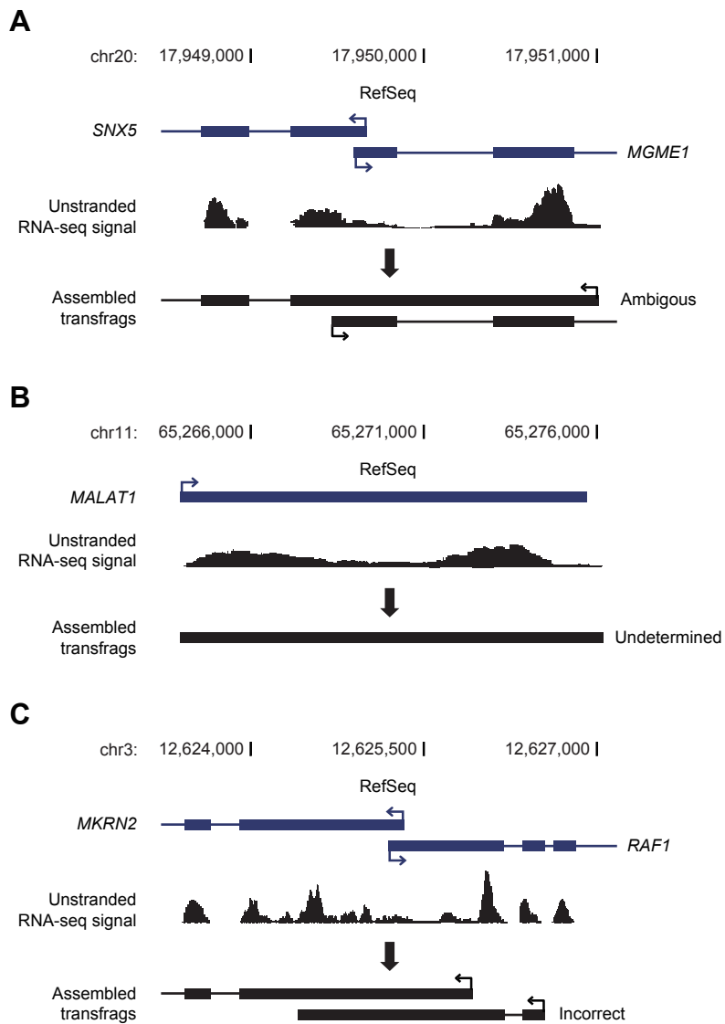
Figure S3. Problematic transfrags assembled from unstranded RNA-seq
