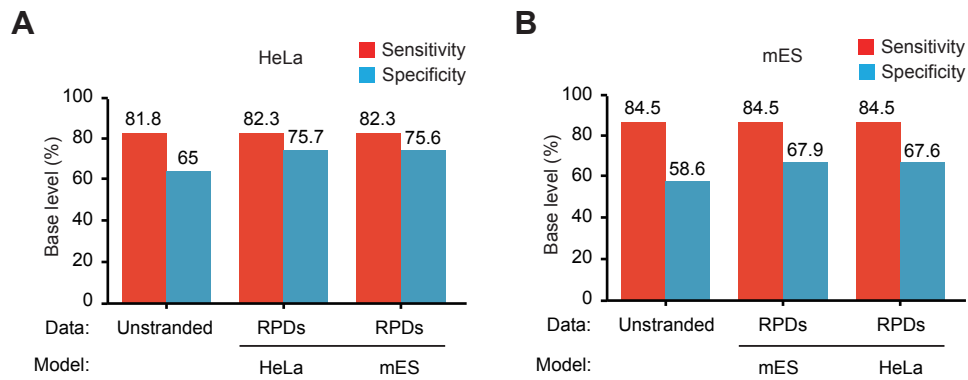
Figure S7. Generality of the kMC model
