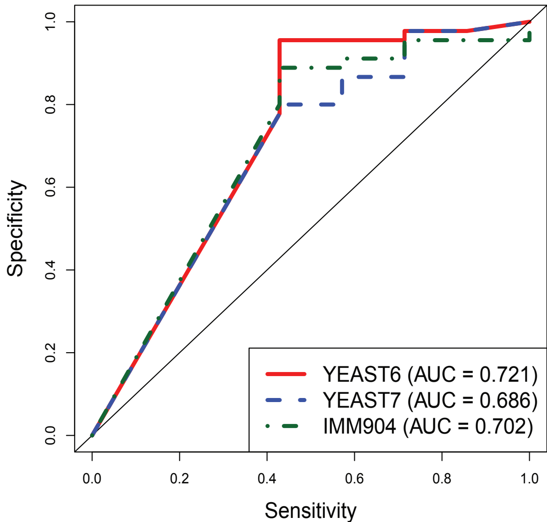
A. Predictions by IDREAM (Threshold=0.5)
