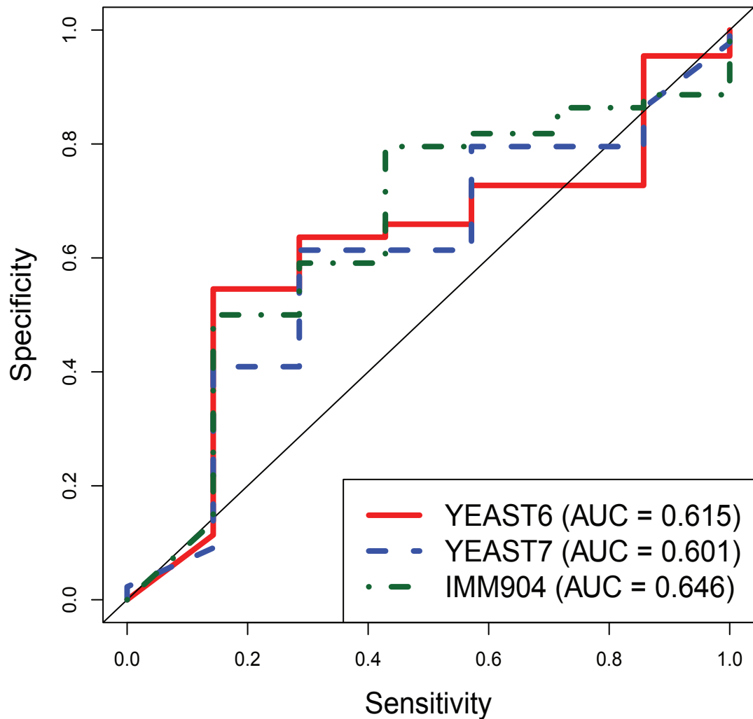
B. Predictions by PROM (Threshold=0.5)
