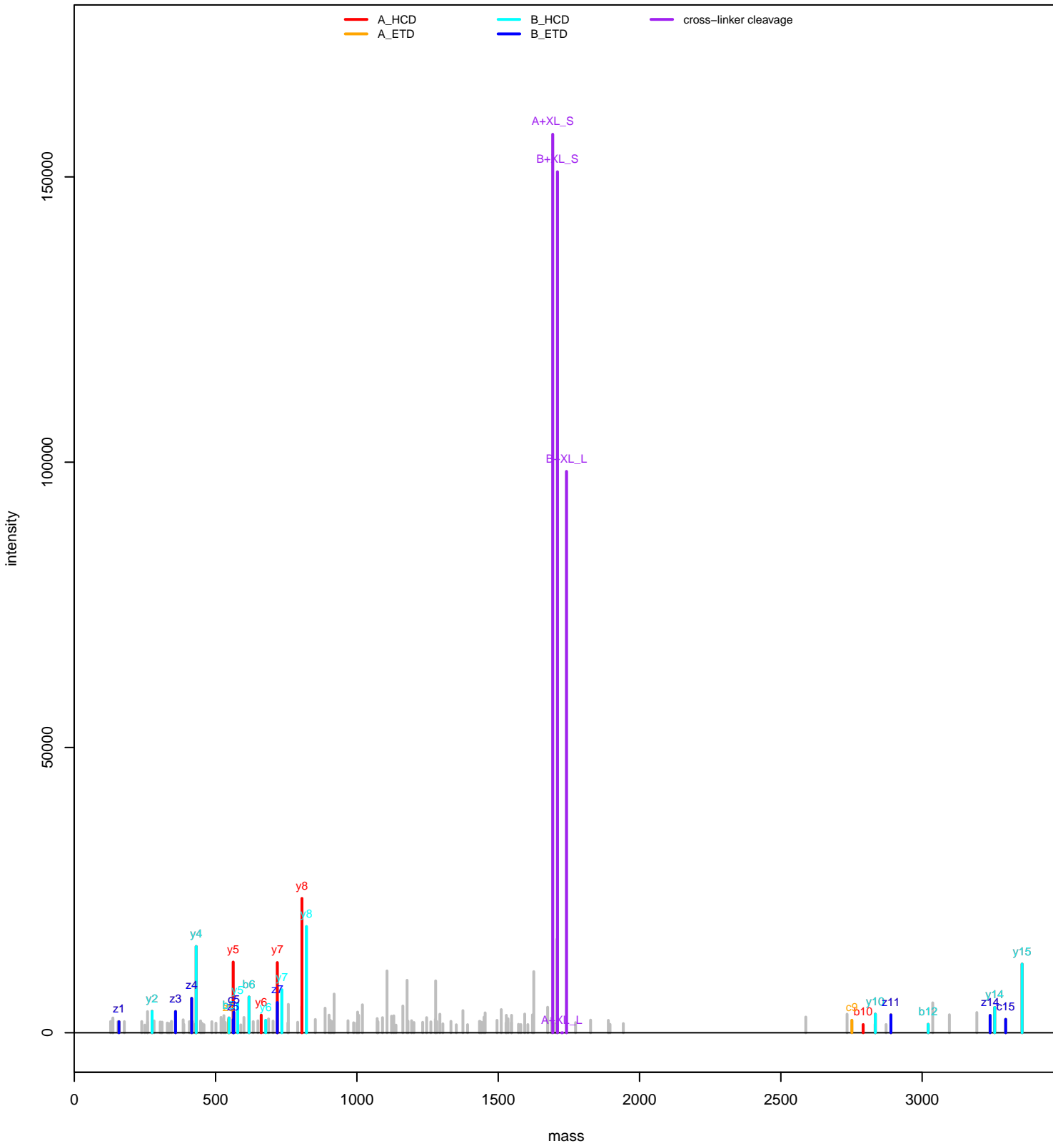
VPSYTASKSGVMGVTR VPSYTASKSGVM o GVTR
