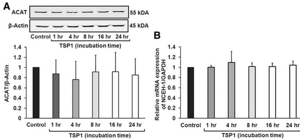
SUPPLEMENTARY FIG. S4. TSP1 does not change ACAT and NCEH-1 expression in macrophages. Macrophages were incubated with vehicle or TSP1 (10 nM) for 1, 4, 8, 16, or 24 h. ACAT protein (Abcam) (A) and NCEH-1 mRNA expression (Bio-Rad) (B) was determined by Western blot and RT-PCR, respectively ( n=3 ). Data represent the mean \pm SD. ACAT, acyl-CoA:cholesterol O-acyltransferase.
