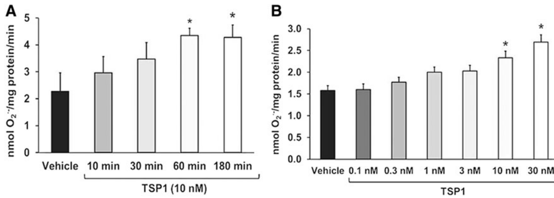
SUPPLEMENTARY FIG. S7. TSP1 time- and concentration-dependently stimulates O 2 - generation in macrophages. (A) RAW 264.7 macrophages were incubated with vehicle (60 min) or 10 nM TSP1 for 10, 30, 60, and 180 min. Superoxide production was measured via cytochrome c reduction. * p < 0.05 versus vehicle ( n = 3). (B) Macrophages were incubated with vehicle or TSP1 (0.1, 0.3, 1, 3, 10, or 30 nM) for 60 min. Superoxide production was measured via cytochrome c reduction. * p < 0.05 versus vehicle ( n = 4–5).
