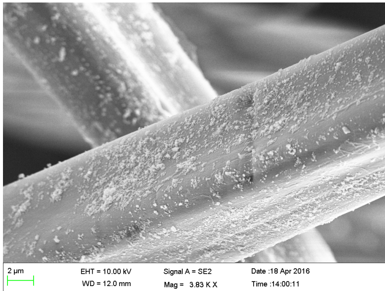
Figure S1. SEM of Ag-Fe 3 O 4 -Silk fiber (2#).
