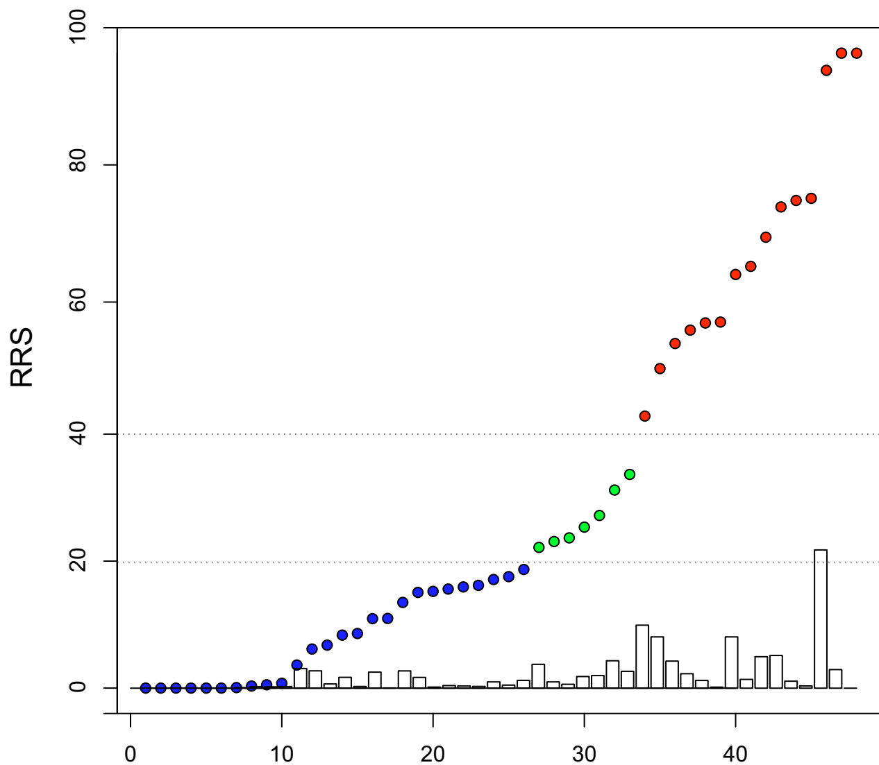
Supplementary Figure 7. Distribution of RRS and cut-off scores for stratification of patients in training cohort. Closed circles represent RRS of each patient and bar graph represents interval of RRS between patients as indicated. First cut-off (40) was chosen between two patients with largest interval of RRS. Second cut-off (20) was chosen between two patients with largest interval of RRS among those with RRS less than 40. Intervals too closed to 0 or 100 were excluded from analysis.
