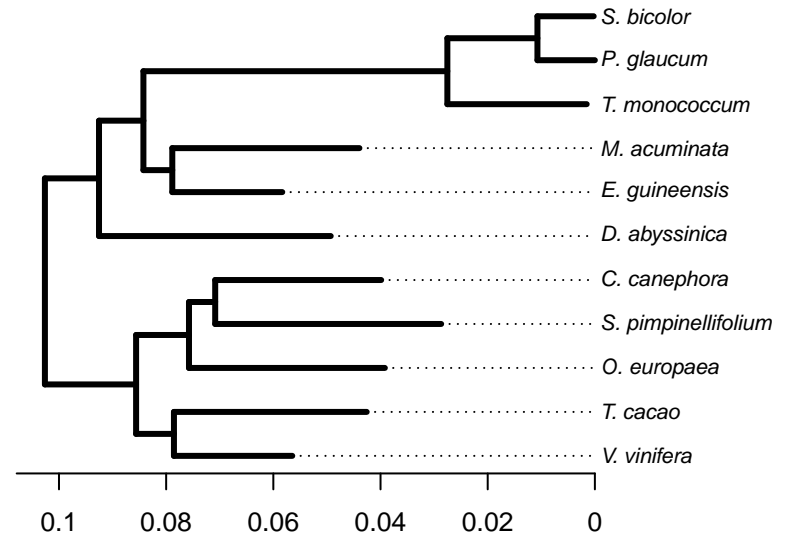
branch lengths = dN
