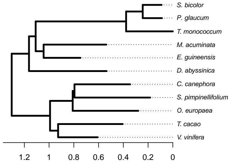
branch lengths = dS
