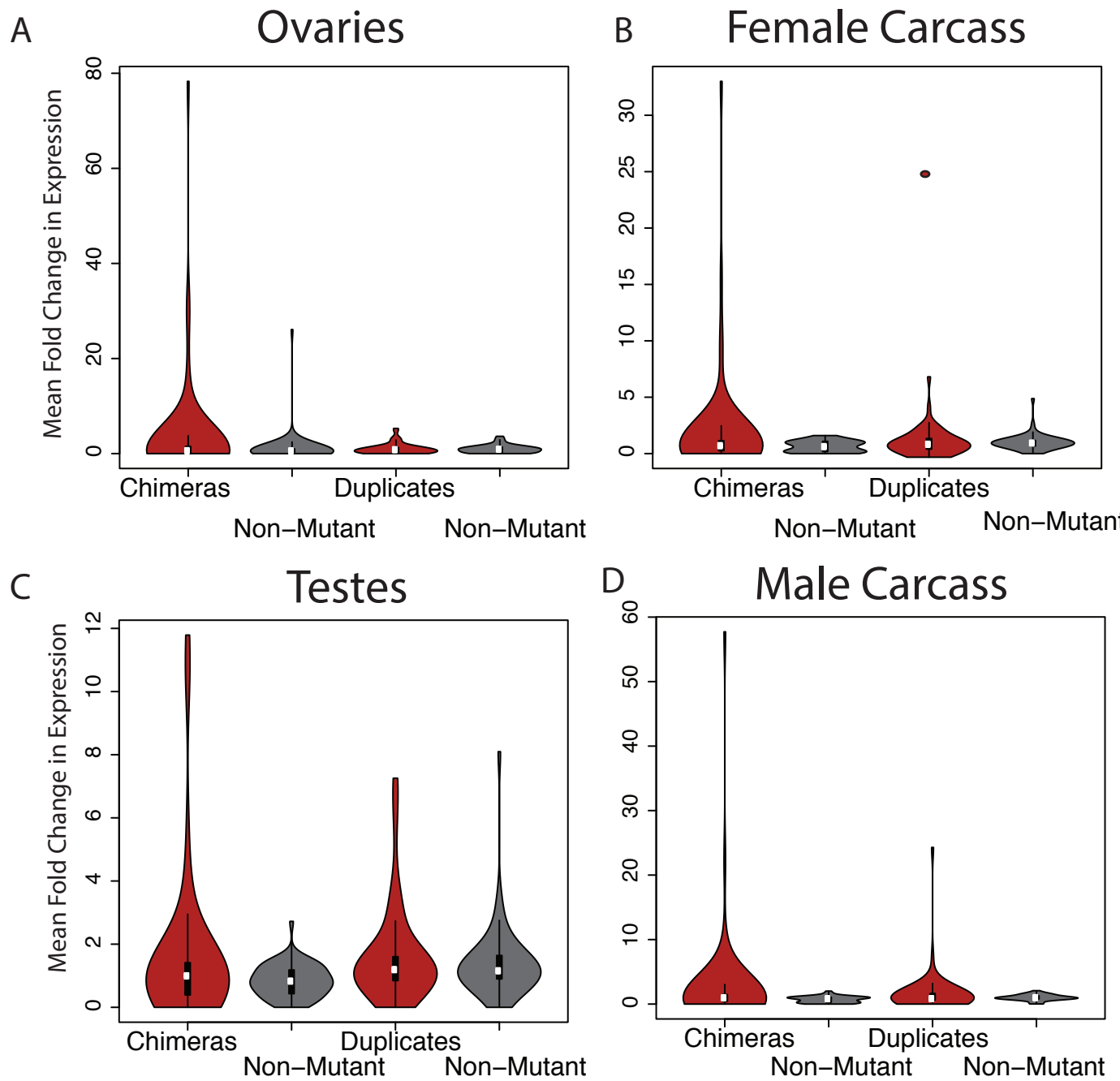
S1 Figure: Mean fold change for chimeric genes in sample strains vs. reference for strains containing chimeras or whole gene duplicates (red) and unmutated sample strains for the same regions (grey). Chimeric genes are more likely to result in high mean fold change than unmutated counterparts in all tissues. Whole gene duplicates create multifold expression changes more rarely.
