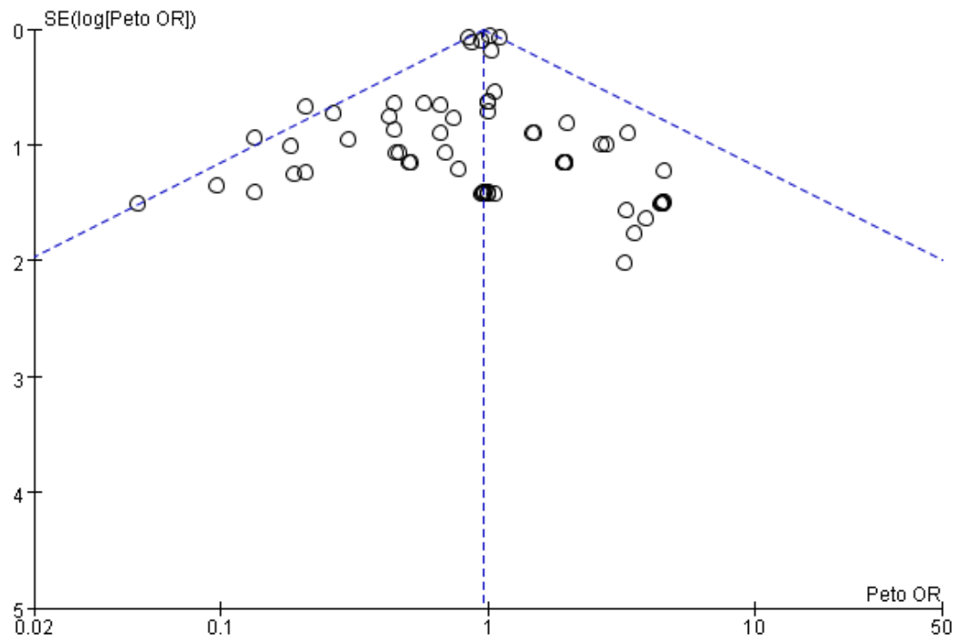
Figure A. Funnel plot of randomised controlled trials reporting all cause mortality among patients receiving incretin versus control
