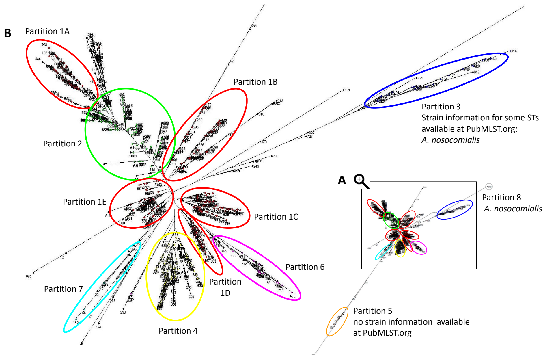
Supp. Fig.1: Partitions as determined by BAPS mapped onto a radial phylogram generated by FastTree 2. (A) Overview and (B) Zoom into the central part of the tree. BAPS partition 1 was further subdivided manually into five subgroups (1A - 1E) according to the branching of the tree. STs that have significant admixture are colored in black.
