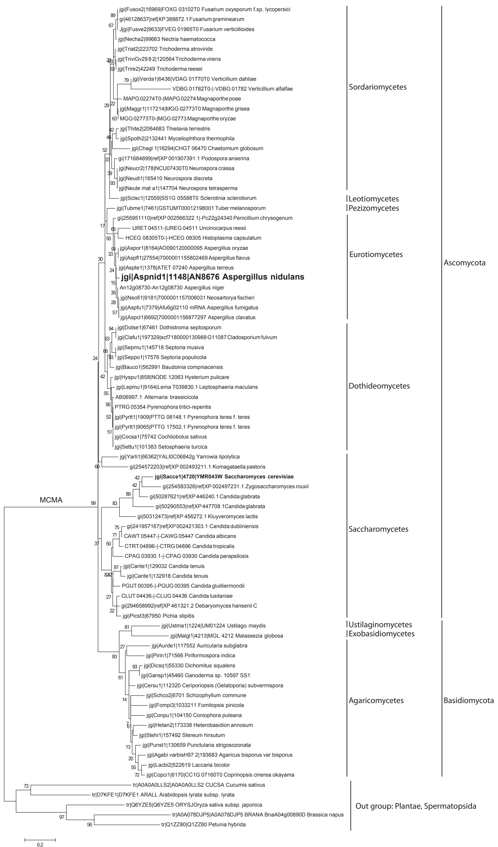
Additional File 4. Maximum likelihood tree of MADS BOX (McmA) Transcription Factors (TFs).
