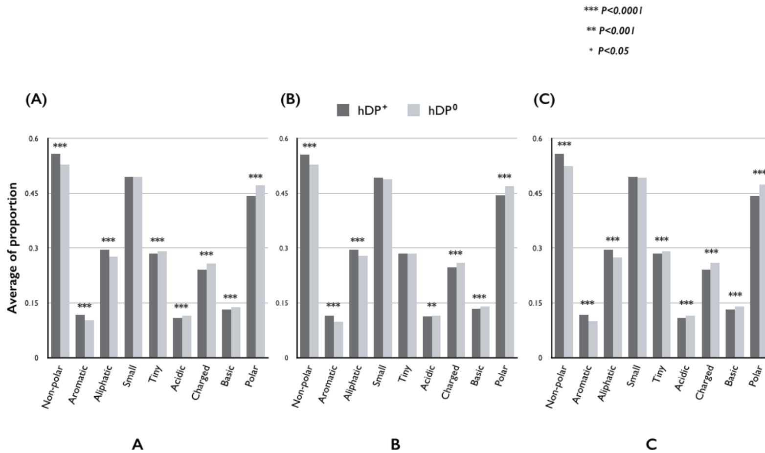
Supplementary Figure 1. Result for amino acid group: (A) for set A. (B) for set B. (C) for Set C.
