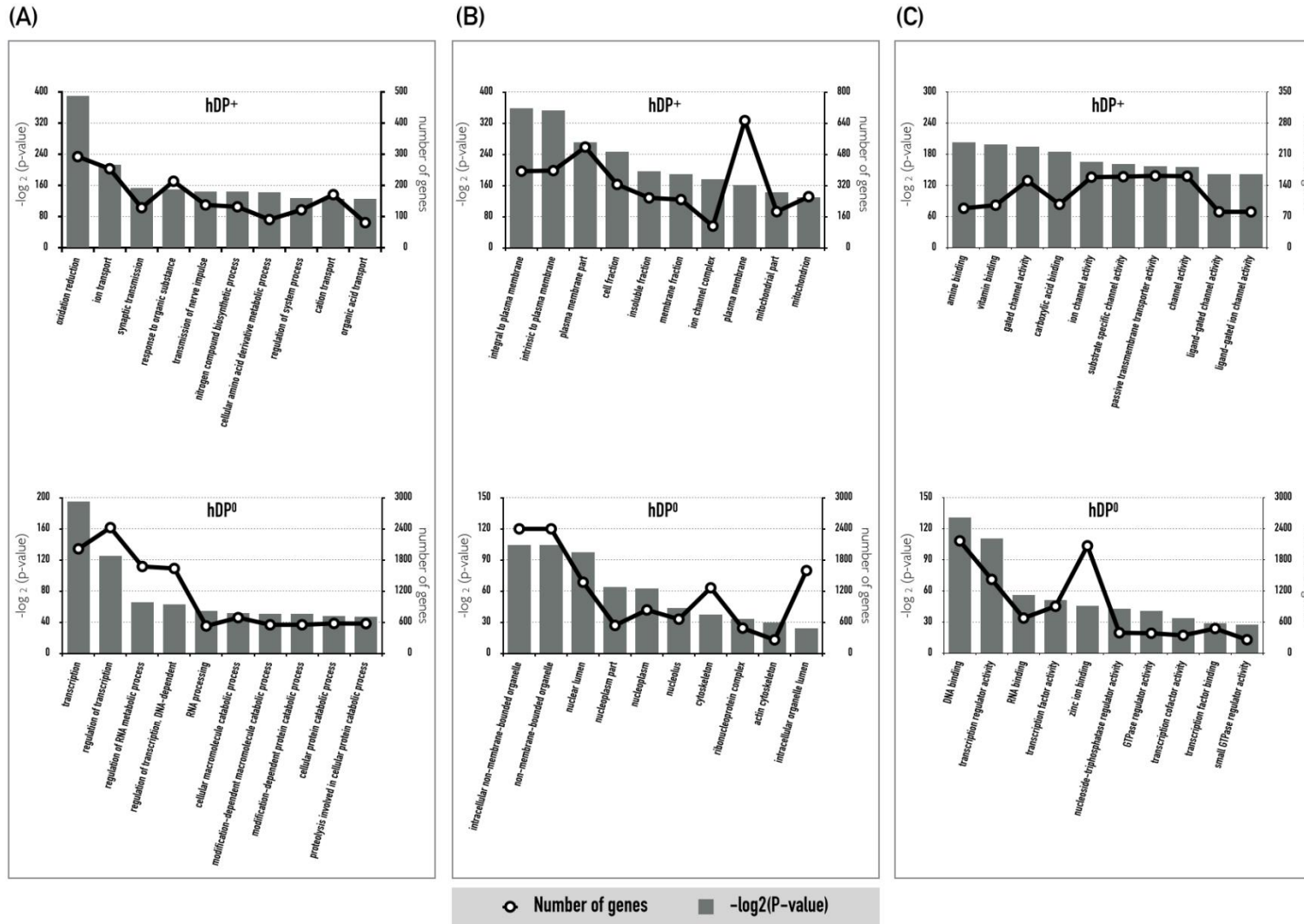
Supplementary Figure 4. Result of gene ontology annotation for set A: (A) Biological processes. (B) Cellular component. (C) Molecular function.
