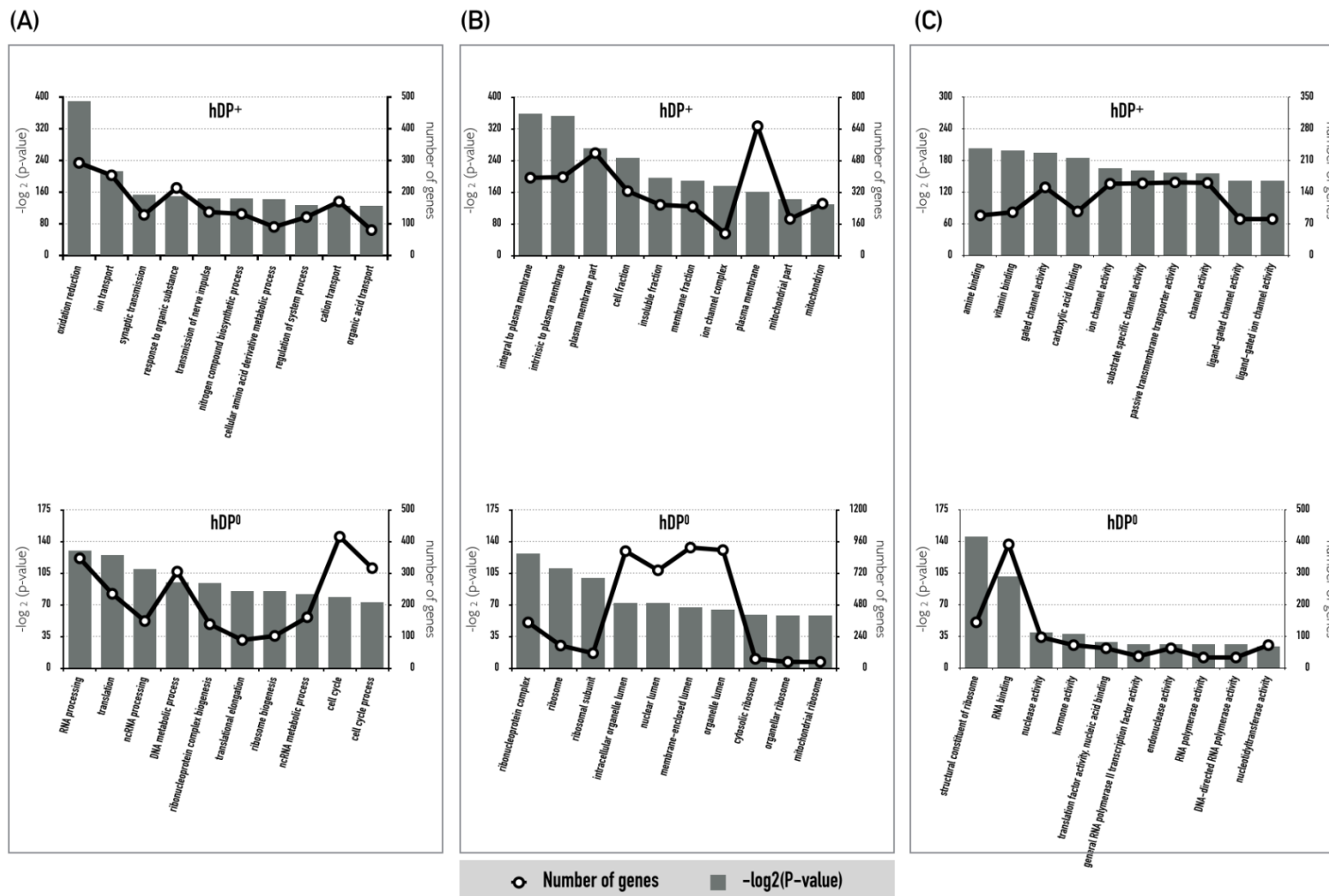
Supplementary Figure 5. Result of gene ontology annotation for set B: (A) Biological processes. (B) Cellular component. (C) Molecular function.
