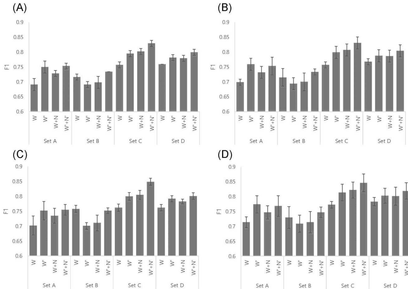
Supplementary Figure 7. 10-fold cross-validation and 10X10 cross-validation with standard derivation. (A) 10-fold cross-validation for SVM. (B) 10-fold cross-validation for RF. (C) 10X10 fold cross-validation for SVM. (D) 10X10 fold cross-validation for RF.
