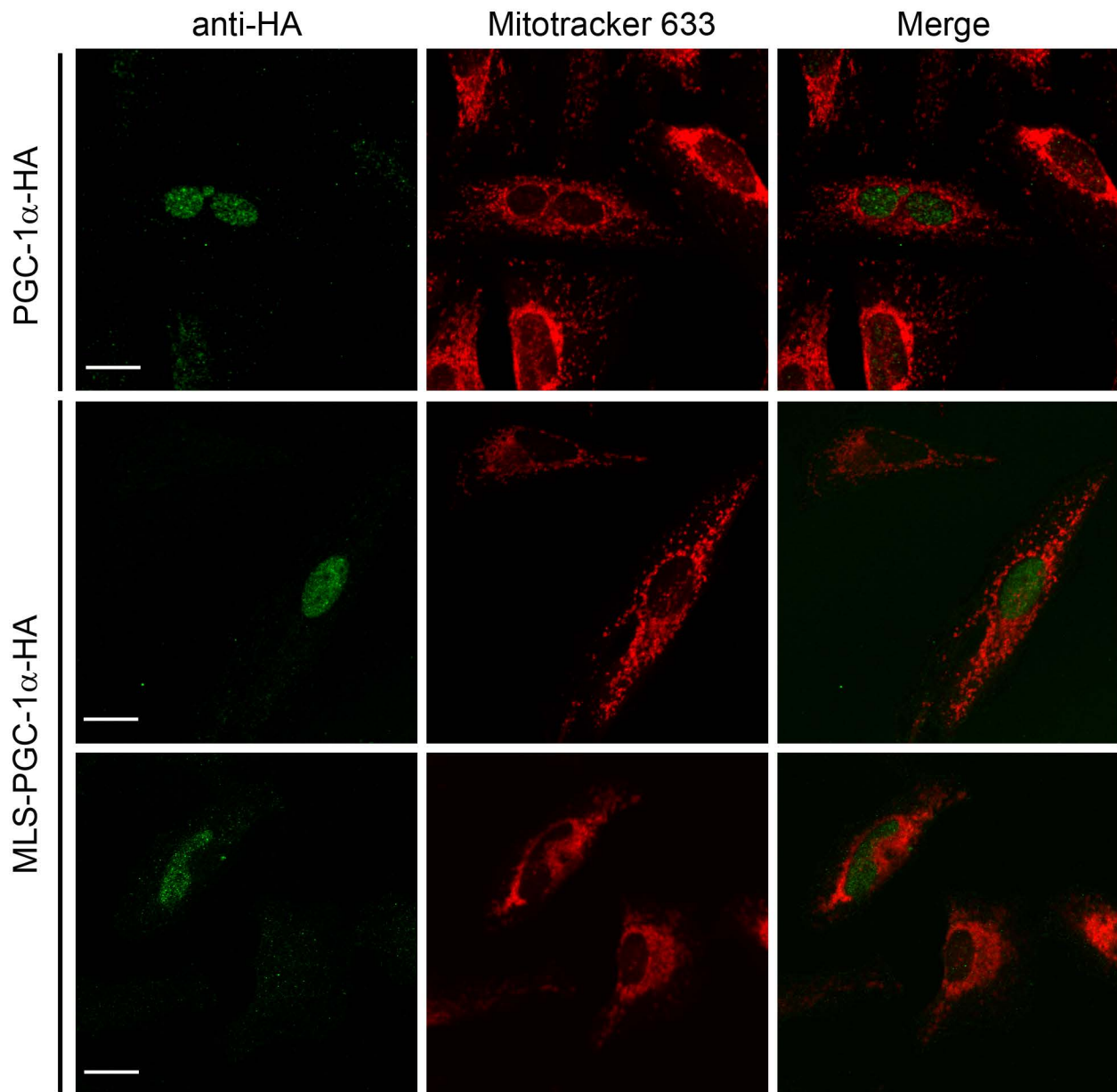
Figure S1. MLS-PGC-1 \alpha localizes in the nucleus.
