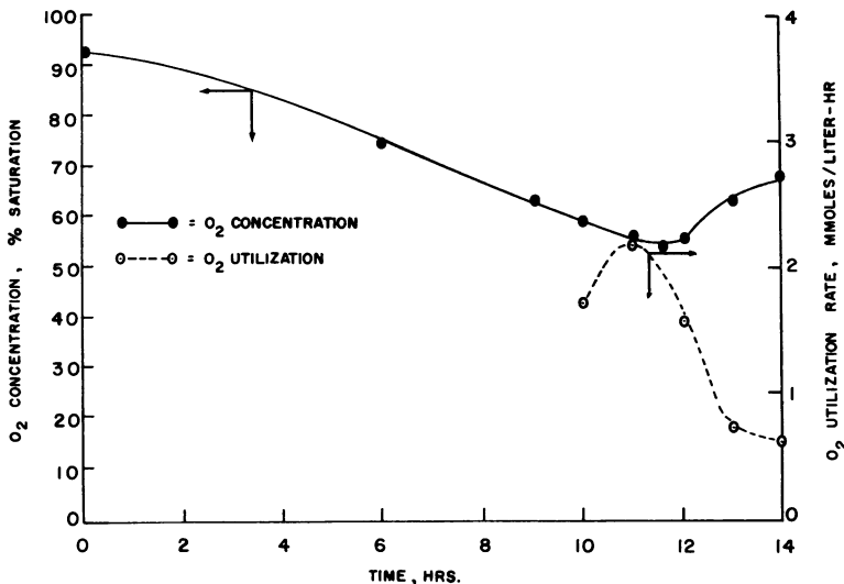
FIG. 4. O_2 concentration and O_2 utilization versus time in N-Z-Amine Type A and glucose medium, pH 6.6.
