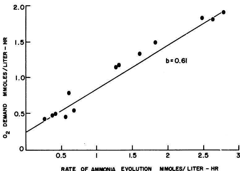
FIG. 6. Oxygen demand versus rate of ammonia evolution per unit cell mass (optical density units).
