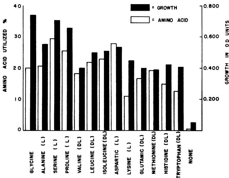
FIG. 5. Percentage amino acid utilization by Pasteurella tularensis LVS (growth in optical density units). (Trace amounts of amino acids present in the yeast supplement account for the values registered by the last set of bars.)
