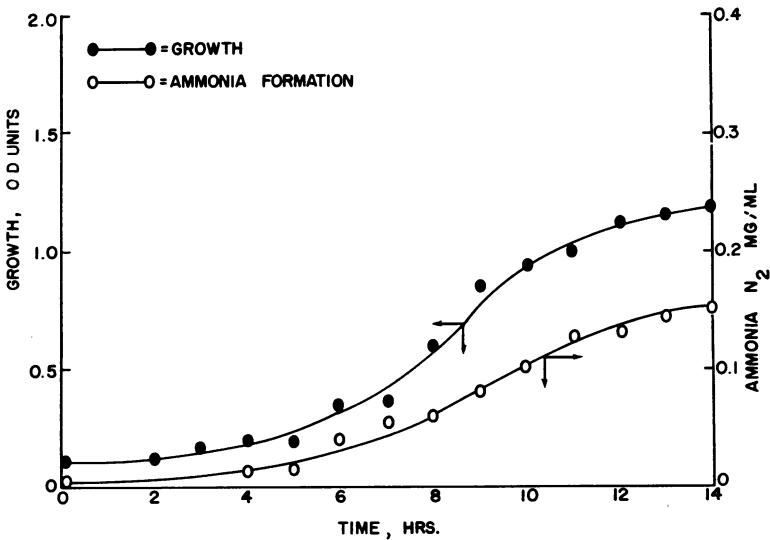
FIG. 3. Growth of Pasteurella tularensis LVS and ammonia formation in N-Z-Amine type A-glucose medium, pH 6.6. (Growth in optical density units.)
