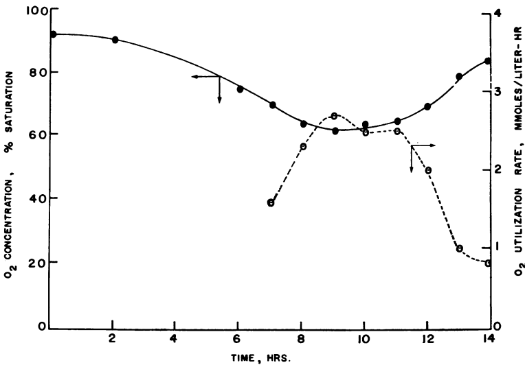
FIG. 2. O 2 concentration and O 2 utilization versus time in casein acid digest and glycerol medium, pH 6.6.
