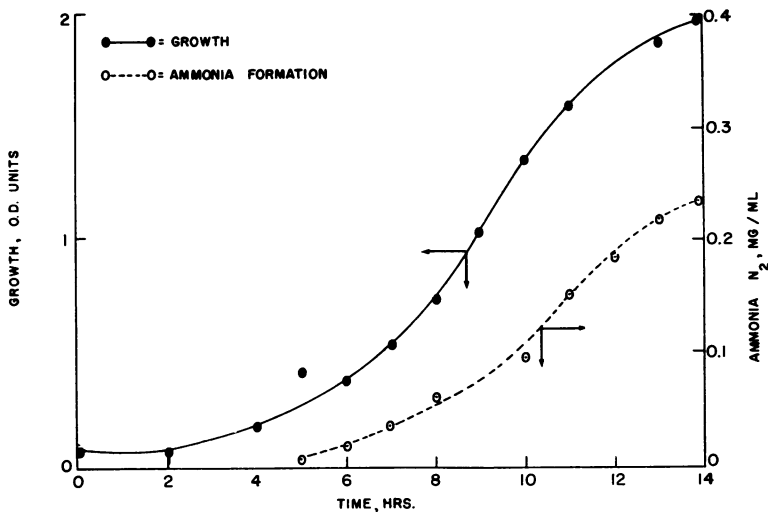
FIG. 1. Growth of Pasteurella tularensis LVS and ammonia formation in casein acid digest and glycerol medium, pH 6.6. (Growth in optical density units.)
