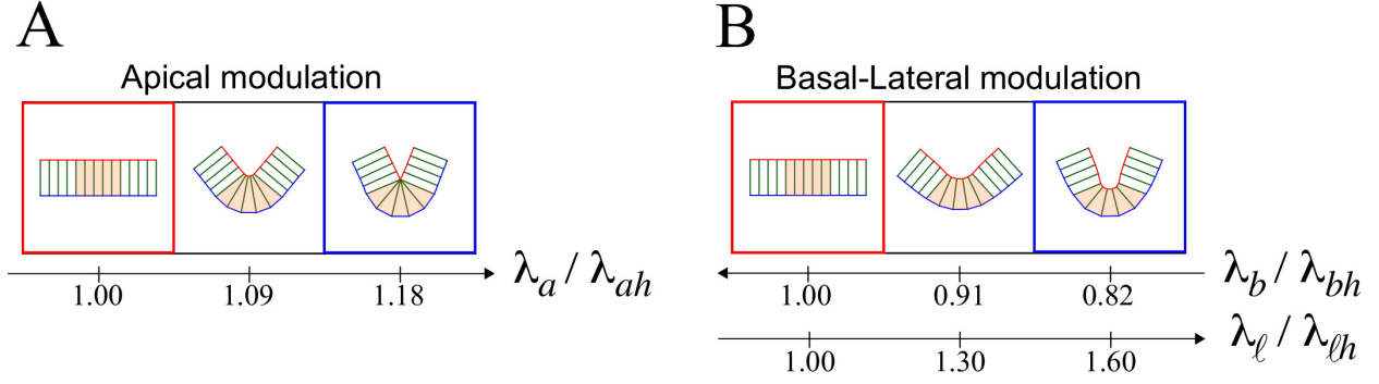
FIG. S4. Epithelial folding for the linear line tension model, where the apical mechanics is described by the line tension \lambda_a . The cells at the center ( N_c = 5 , colored by orange) of the sheet ( N = 13 ) are mechanically modulated at the apical (A) or basal-lateral (B) surfaces. The flat sheet (red box) is generated at parameter values as those shown at the center of Fig. 1C with \lambda_a = \lambda_b . Note that the different modulation mechanisms sculpt epithelia into distinct folds (blue box) similar to those observed in our model considering the effect of apical elasticity.
