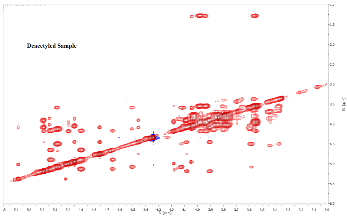
Figure S2. 2D TOCSY spectra of native and deacetylated JL2810 EPS.
