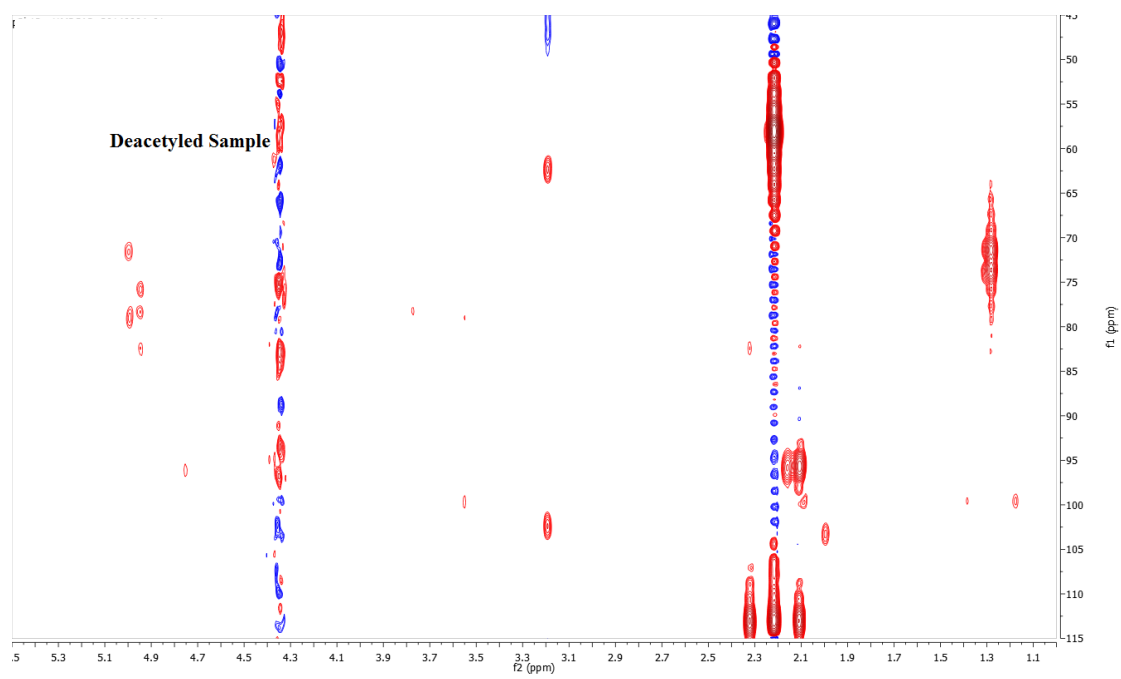
Figure S4. 2D gHMBC spectrum of deacetyled JL2810 EPS.
