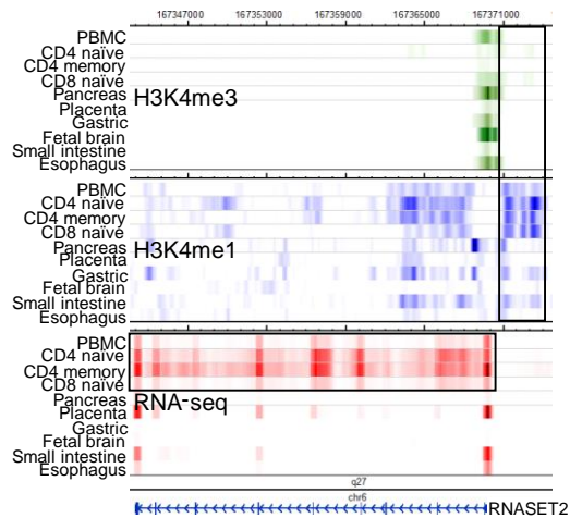
Fig. S5. Tissue-specific functional annotation of RNASET2 locus. Heatmap of H3K4me3, H3K4me1 and RNAseq data from REMC
