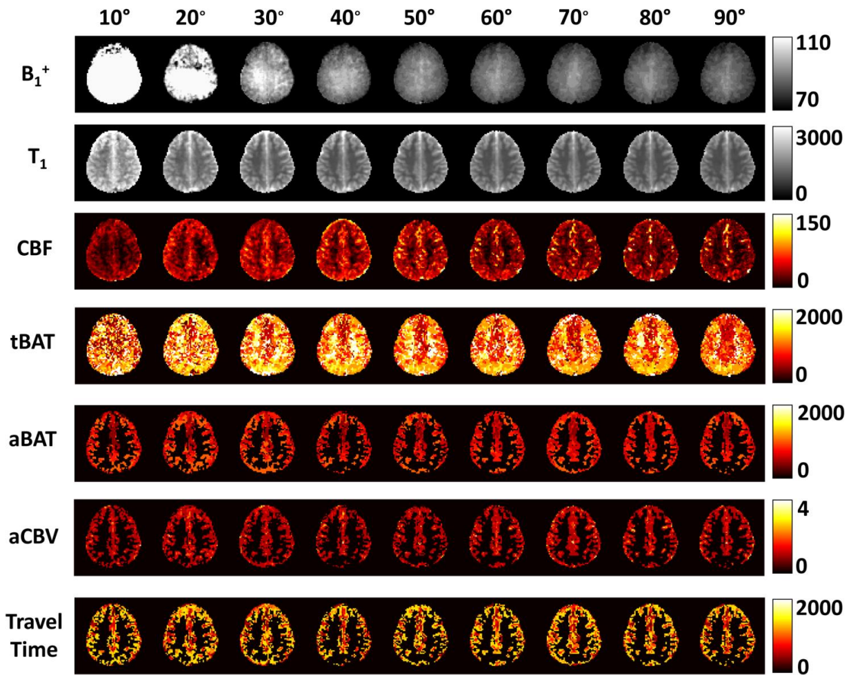
Supporting Figure S1 - Two-compartment MRF-derived parametric maps as a function of flip angle: B_1^+ (%), tissue T_1 (ms), CBF (ml/100g/min), tissue BAT (ms), pass-through arterial BAT (ms), pass-through blood volume (%) and pass-through blood travel time (ms).
