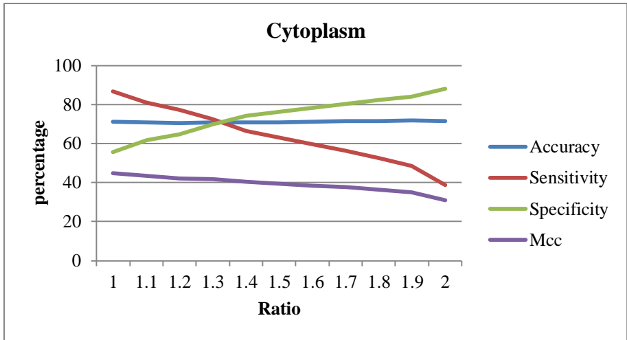
Supplementary figure 4 Negative and positive ratio test in Cytoplasm by SVMs
